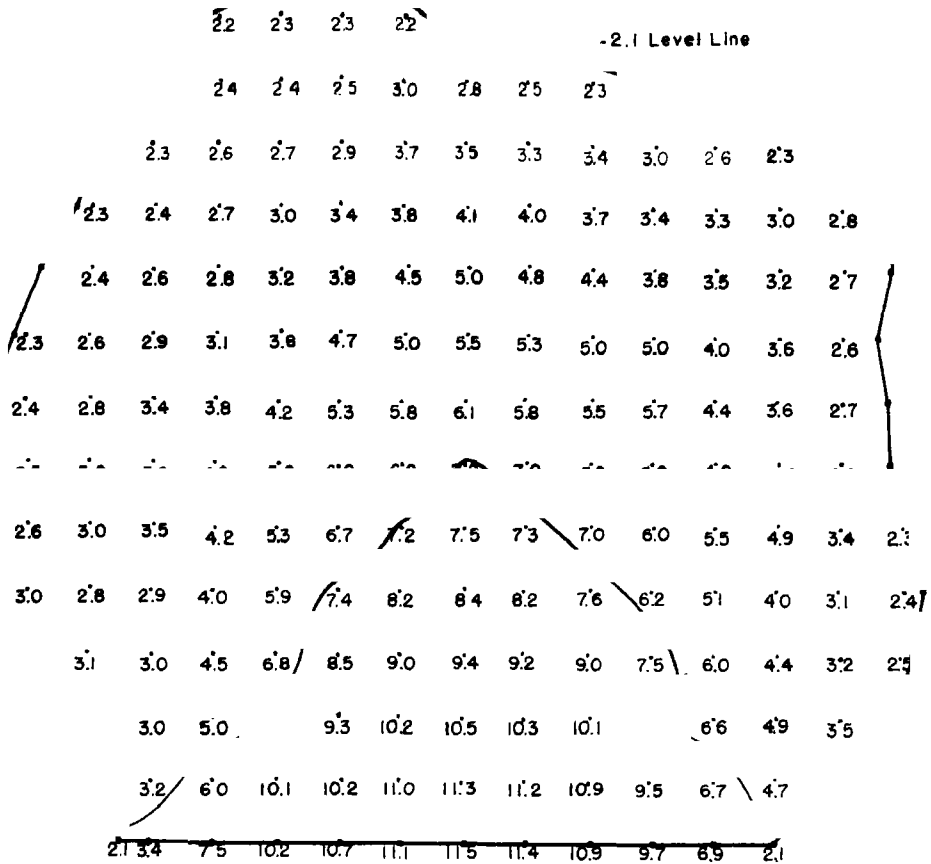
FIGURE 2. Topographic survey of proposed pond area, showing levels of natural ground at ten-foot intervals (compared to water line at 2.1 feet). Area below "A" line will become shallower due to fill. Area within "B" line is deepest, being over five feet prior to any excavation.
