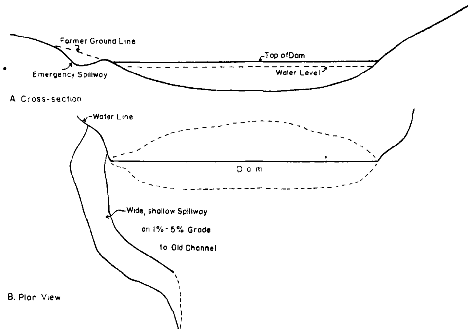
FIGURE 6. Emergency Spillway.
