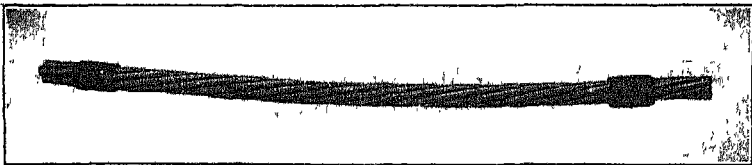
FIG. 124.—PIECE OF SUPPORTING STRAND.
