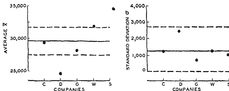
FIG. 110.—CONTROL CHART FOR SMALL SAMPLES SHOWING LACK OF CONTROL.
