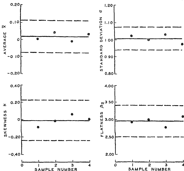
FIG. 109.—CONTROL CHART TEST APPLIED TO CONTROLLED DATA GIVES CONSISTENT RESULTS.
