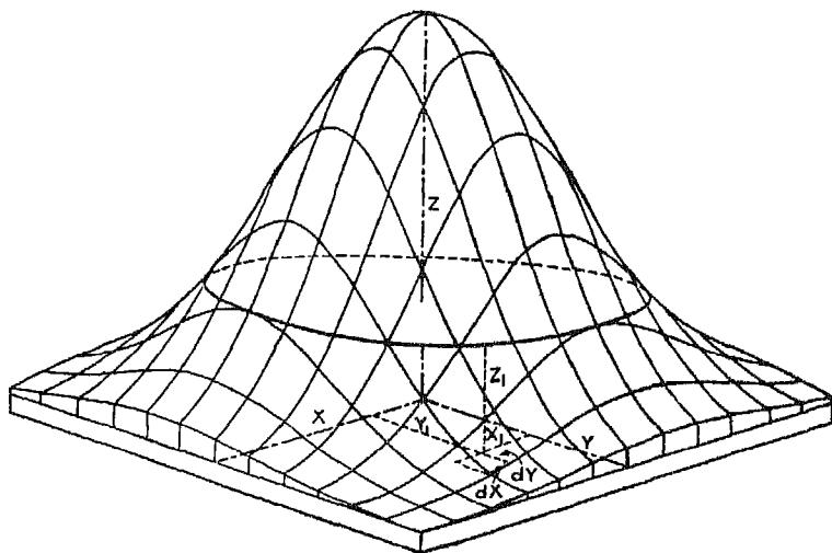
FIG. 35.—THE NORMAL SURFACE.
