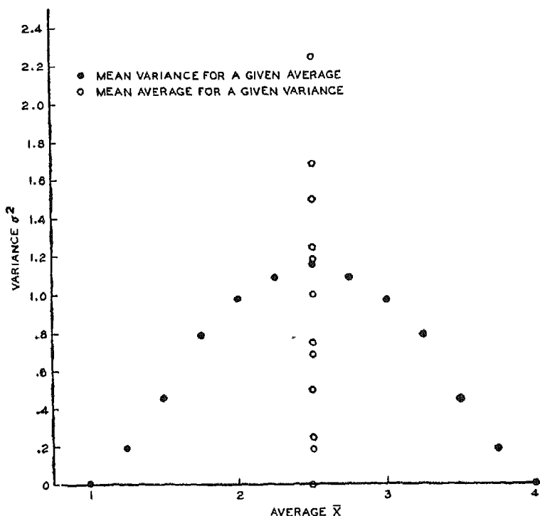
FIG. 66.—SCATTER DIAGRAM FOR AVERAGES AND VARIANCES OF ALL POSSIBLE SAMPLES OF FOUR FROM UNIVERSE I, 2, 3, 4.
