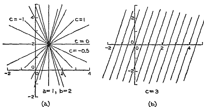
FIG. 34.—GRAPH OF FUNCTION Y = c(X - a) + b SHOWING SIGNIFICANCE OF PARAMETERS a , b , AND c .
