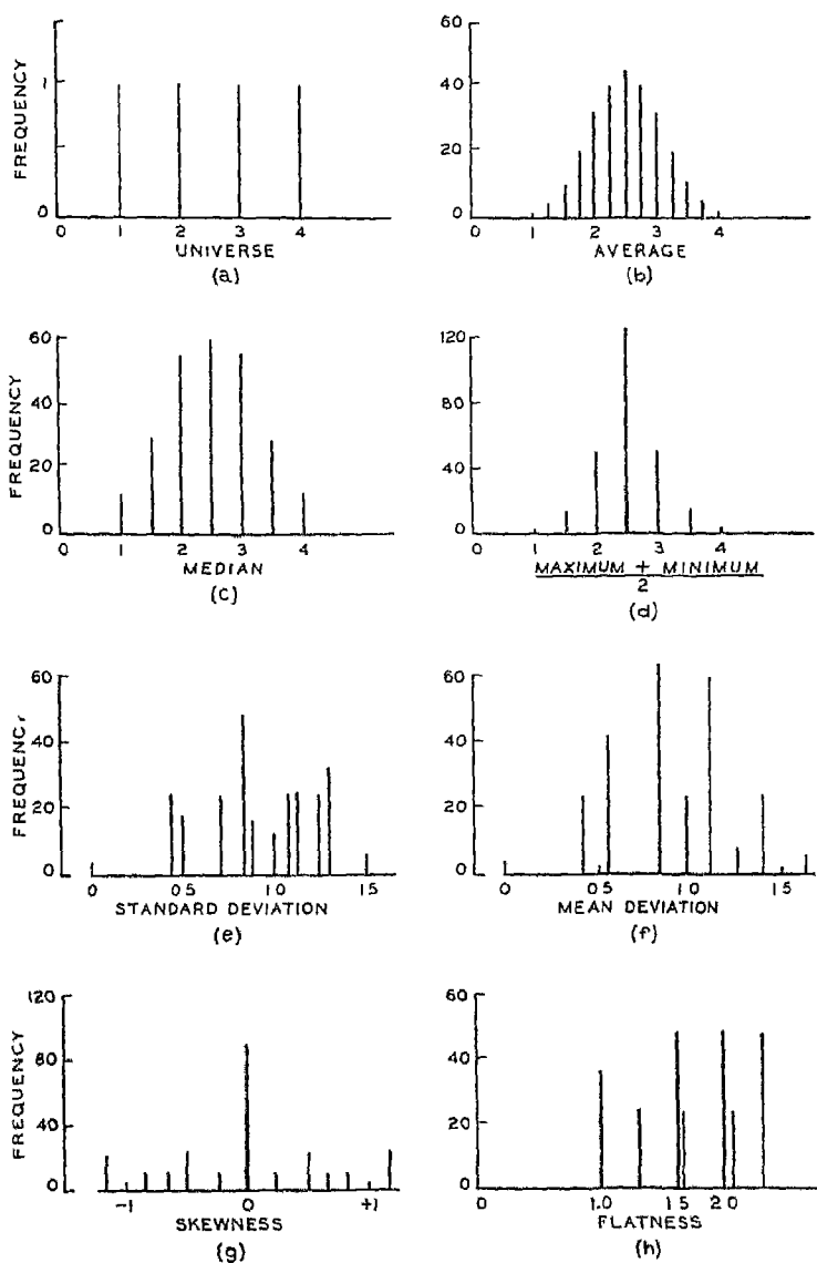
FIG. 57.—DISTRIBUTION OF STATISTICS FOR SAMPLES SHOWN IN TABLE 25.
