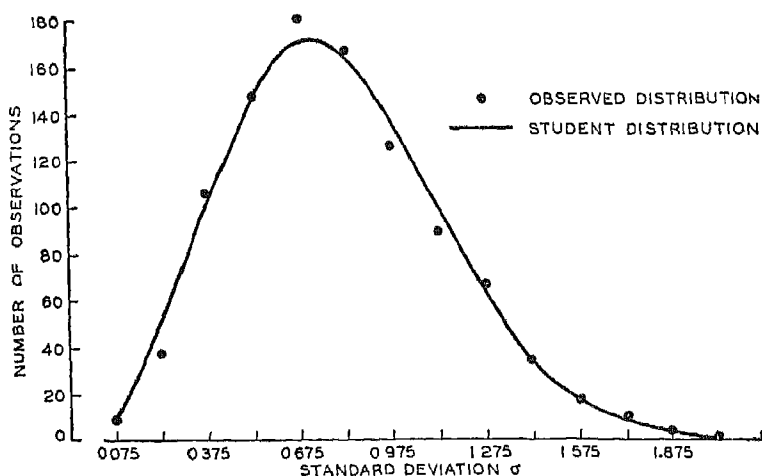
FIG. 60.—DISTRIBUTION OF STANDARD DEVIATIONS IN SAMPLES OF FOUR DRAWN FROM NORMAL UNIVERSE
