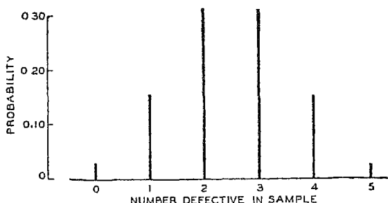
FIG. 121.—CONSUMER'S RISK.
