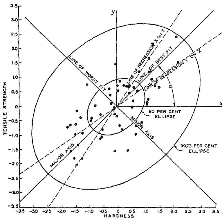
FIG. 40.—INFORMATION GIVEN BY AVERAGE, STANDARD DEVIATION, AND CORRELATION COEFFICIENT.
