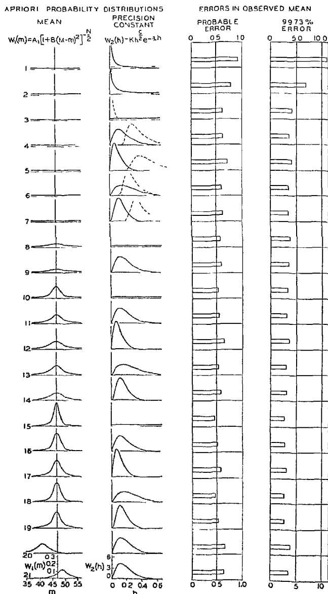
FIG. 130.—SIGNIFICANCE OF a priori EXISTENCE PROBABILITY FUNCTIONS.
