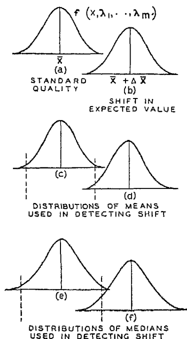
FIG. 94.—ILLUSTRATING IMPORTANCE OF PROPER CHOICE OF STATISTICS.
