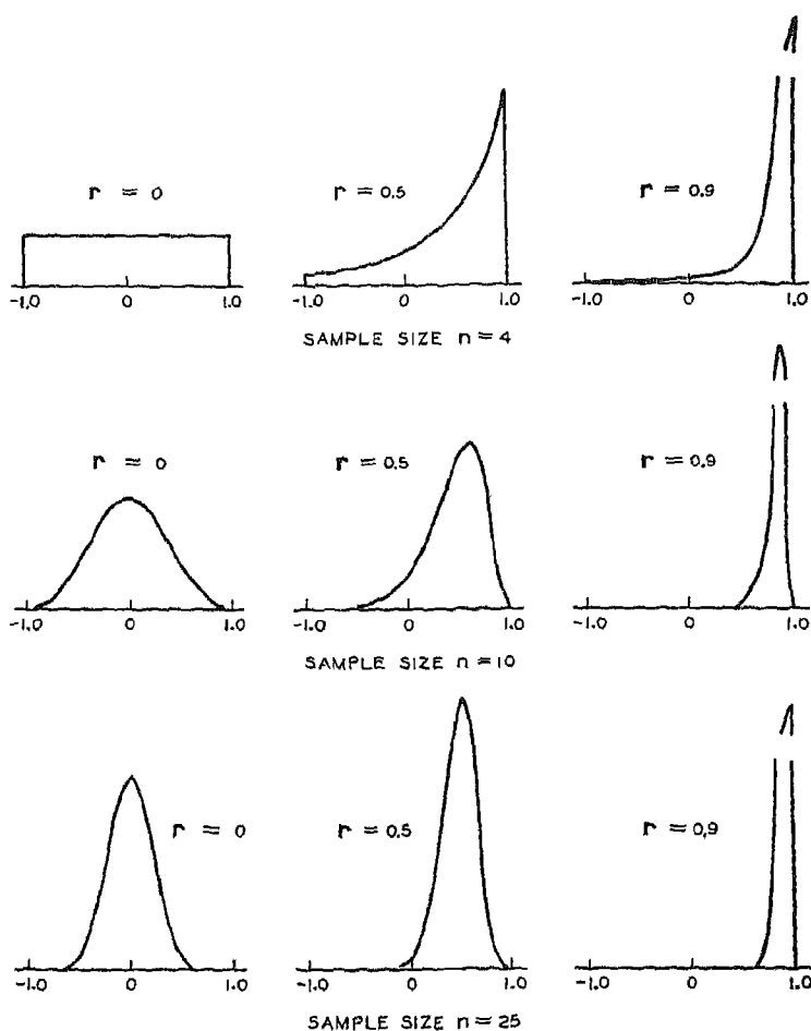
FIG. 76.—TYPICAL DISTRIBUTIONS OF CORRELATION COEFFICIENT.
