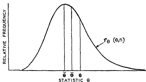
FIG. 97.—SCHEMATIC ASYMMETRICAL DISTRIBUTION OF A STATISTIC.
