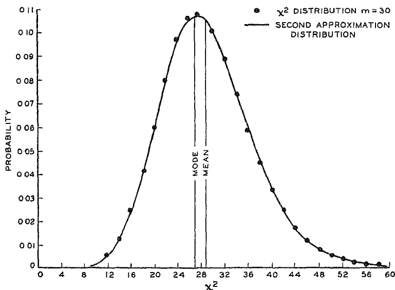
FIG 74 — DISTRIBUTION OF \chi^2 FOR m = 30
