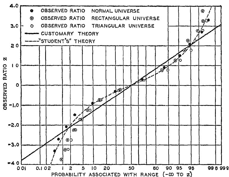
FIG. 63—PROBABILITY ASSOCIATED WITH RANGE (-\infty \text{ to } z) .
