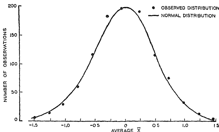
FIG. 58—EXPERIMENTAL EVIDENCE THAT THE DISTRIBUTION OF AVERAGES OF SAMPLES OF SIZE n DRAWN FROM AN EXPERIMENTALLY NORMAL UNIVERSE IS NORMAL.
