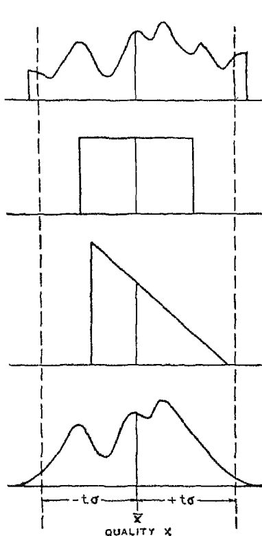
FIG. 92.—FOUR UNIVERSALS OF EFFECTS SATISFYING THE SPECIFICATION THAT THE EXPECTED VALUE SHALL BE \bar{X} AND STANDARD DEVIATION SHALL BE \sigma .
