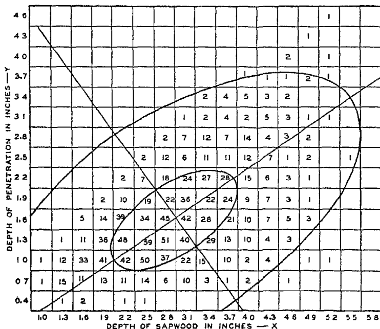
FIG. 39.—ILLUSTRATION OF METHOD OF FINDING 50 PER CENT AND 99.7 PER CENT ELLIPSES FROM THE DATA
