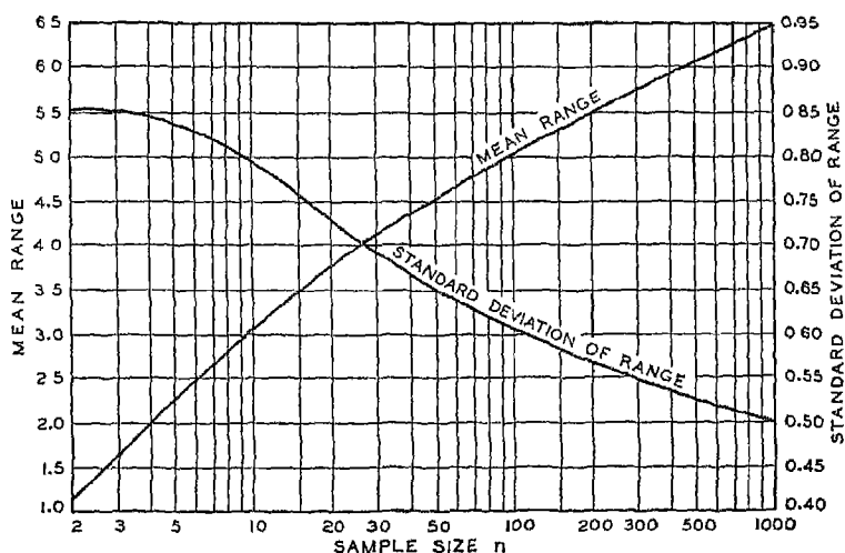
FIG. 70.—THEORETICAL VALUES OF MEAN RANGE AND STANDARD DEVIATION OF RANGE FOR SAMPLES OF SIZE n .
