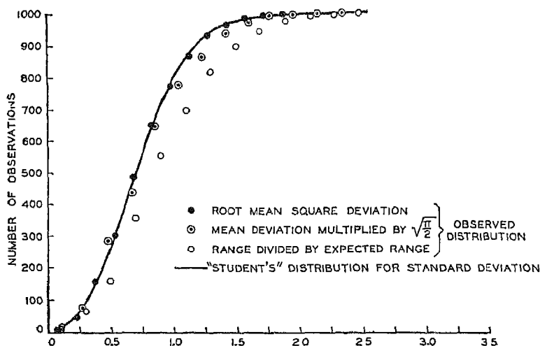
FIG. 71.—DISTRIBUTIONS OF THREE ESTIMATES OF STANDARD DEVIATION OF UNIVERSE.
