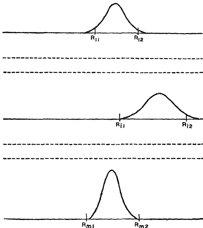
FIG. 86.—TOLERANCE RANGES ON OBSERVED DISTRIBUTIONS.
