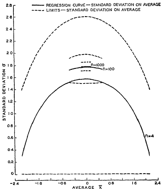
FIG. 102.—EFFECT OF SAMPLE SIZE ON LIMITS.
