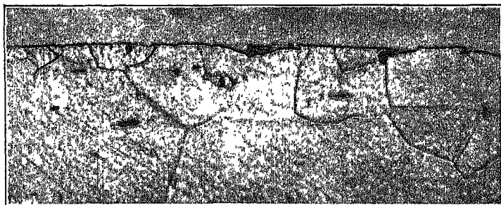
FIG. 146.—TYPICAL CROSS SECTION OF A PROTECTIVE COATING—NOTE IRREGULAR LINE OF DEMARKATION BETWEEN COATING AND METAL.
