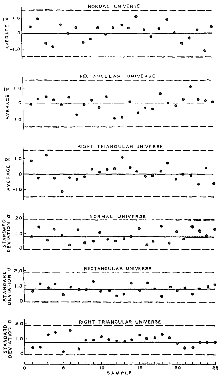
FIG. 112.—CRITERION I APPLIED TO 25 SAMPLES OF 4 FROM EACH OF 3 UNIVERSES—VALUES IN TERMS OF \sigma OF THEIR RESPECTIVE UNIVERSE.
