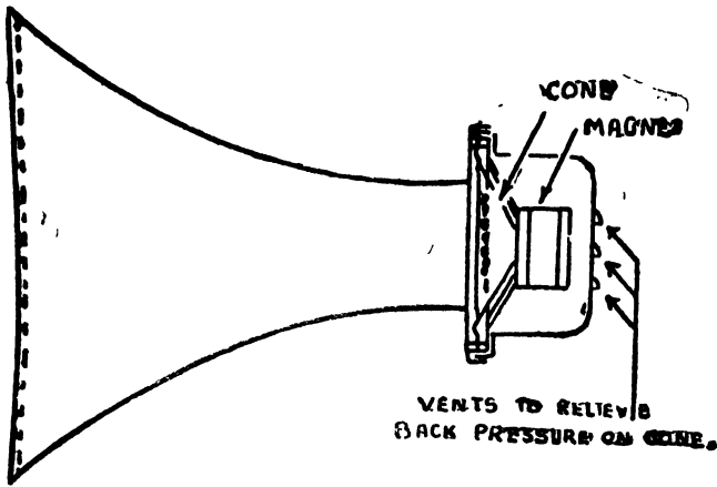
Fig. 28 Loud Speaker.
