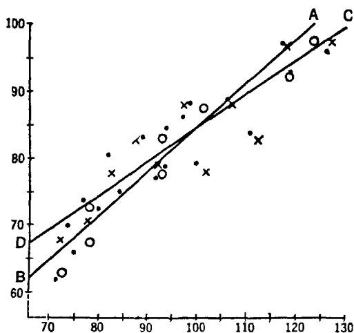
FIG. 39 CORRELATION GRAPH CONTAINING REGRESSION LINES
