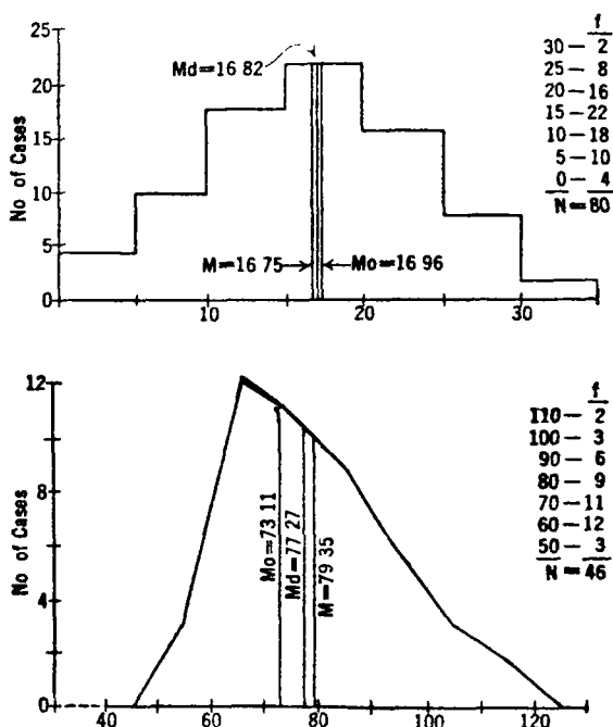
FIG. 29 GRAPHIC REPRESENTATION OF THE MEAN, MEDIAN, AND MODE
