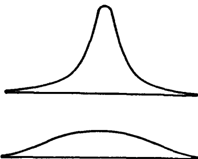
FIG 22 LEPTOKURTIC AND PLATYKURTIC FREQUENCY CURVES
