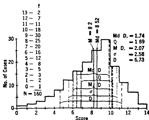
FIG. 33. SKEW CURVE SHOWING MEASURES OF VARIABILITY
