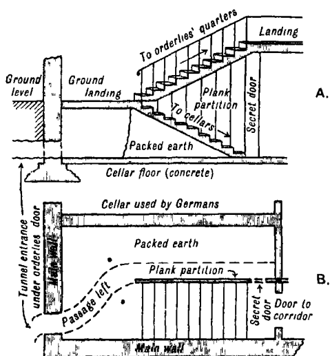
A. Section, B. Ground-plan of staircase, chamber, and tunnel entrance.
