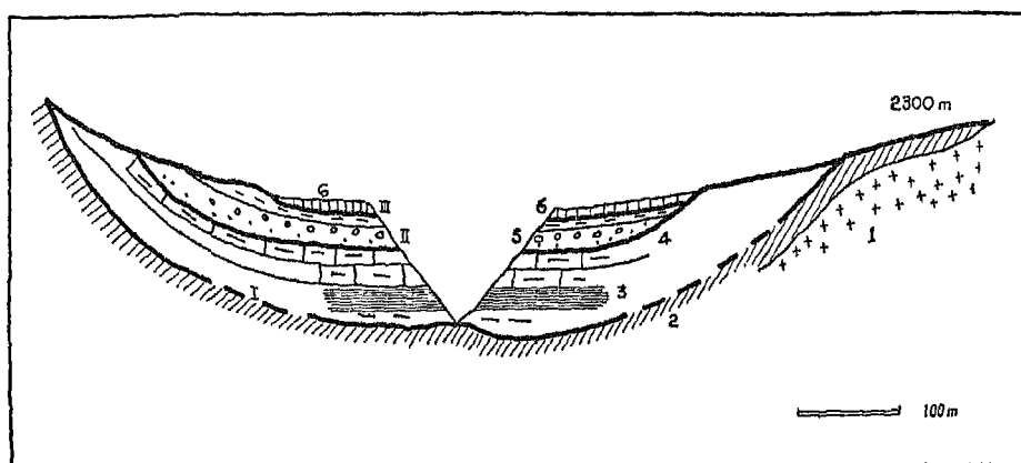
FIG. 8. GENERALIZED CROSS-SECTION THROUGH UPPER ACATLÁN BARRANCA NEAR TEQUIXQUIAC
