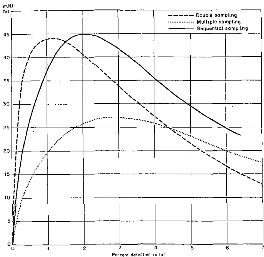
FIG. 6.2.— \sigma(N) curves for double, multiple, and sequential plans of Table 6.1.
