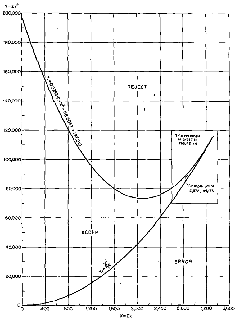
FIG. 1.5.—Graphical procedure for determining from \sum x and \sum x^2 whether \bar{x} + ks \leq U ; N = 95 , k = 0.7645 , U = 35 .
