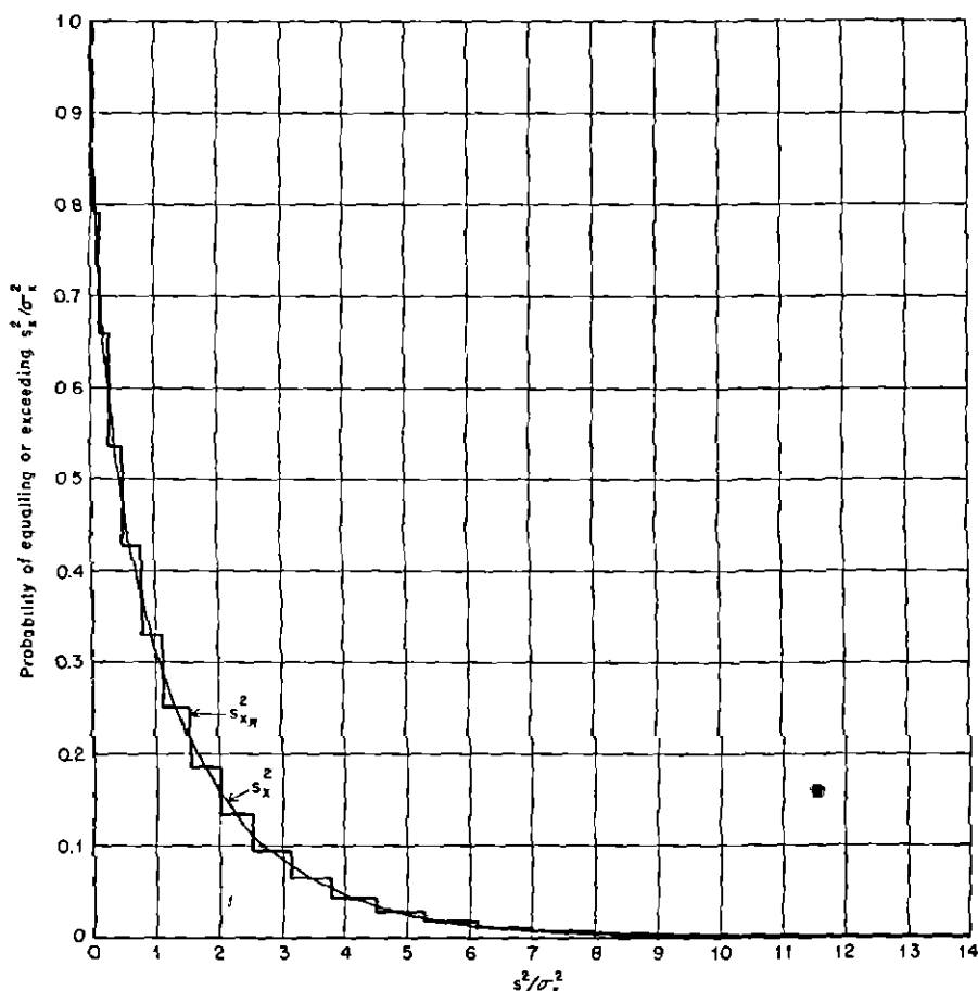
FIG. 4.3.—Distribution of s_{xR}^2 for samples of 2 from a normal population when the width of the rounding interval is one-quarter standard deviation, and corresponding continuous distribution of s_x^2 .
