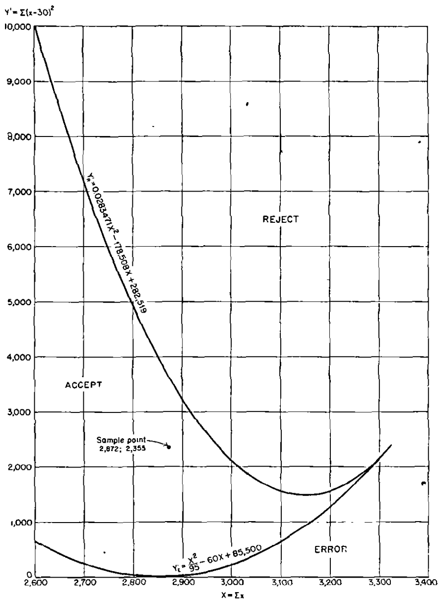
FIG. 1.7.—Graphical procedure for determining from \Sigma x and \Sigma(x - A)^2 whether \bar{x} + ks \leq U ; N = 95 , k = 0.7645 , U = 35 , A = 30 .
