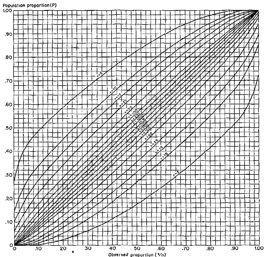
FIG. 10.4.—Eighty percent confidence belts for population proportion.
