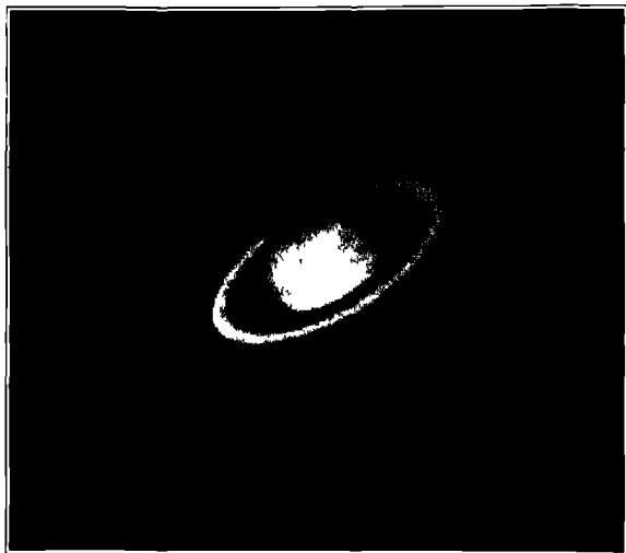
FIG 156 Saturn
