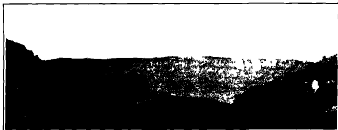
FIG 181 Meteor Crater, Arizona
