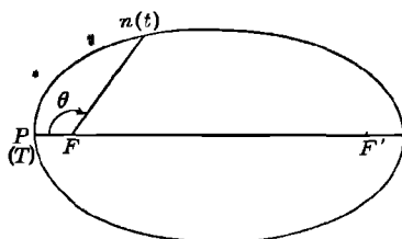
FIG 124 Kepler's Problem
