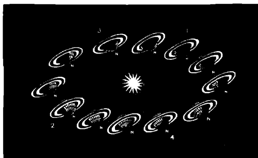
FIG 158 The Phases of Saturn's Rings
