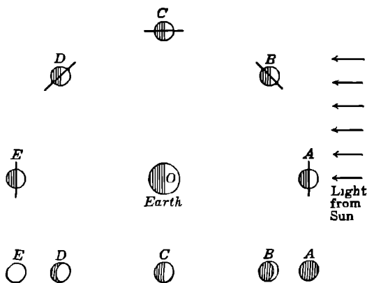
FIG. 69 Phases of the Moon
