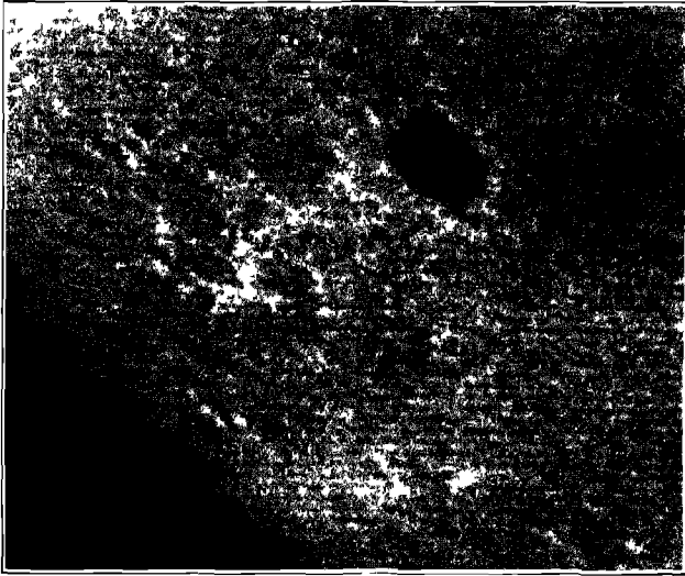
FIG. 90 Single Normal Spot, with Faculae
