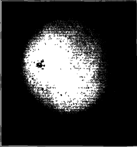
FIG 88 Sun-Spot Maximum
