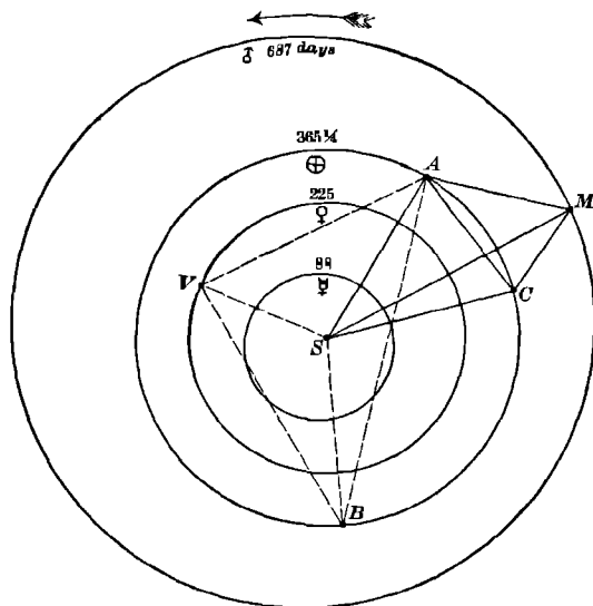
FIG 117 Distance of a Planet
