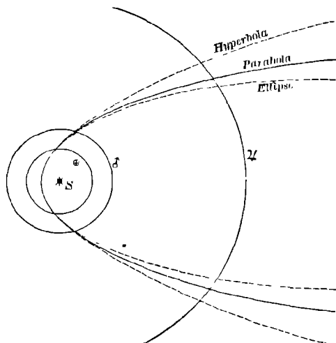
FIG. 164 The Close Coincidence of Different Species of Cometary Orbits within the Earth's Orbit The earth's orbit is indicated by the sign ⊕
