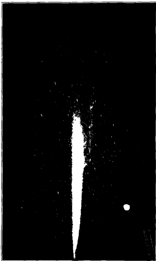
FIG 167 Halley's Comet
