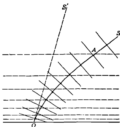
FIG. 44 Refraction of Light in the Earth's Atmosphere
