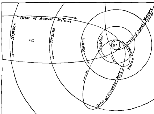
FIG 183 Orbits of Meteoric Swarms
