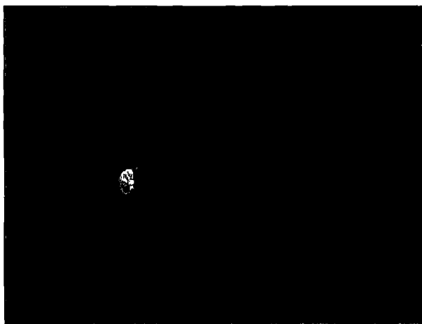
FIG 173 Head of Donati's Comet
