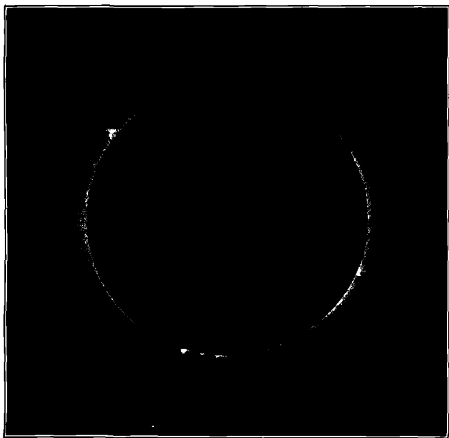
FIG. 107 A The Eclipse of June 8, 1918, Goldendale, Washington
