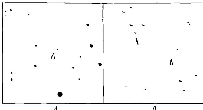
FIG 146 The Asteroid (508) Princeltonia
