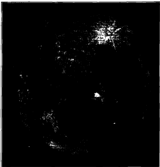
FIG. 81 The Nearly Full Moon
