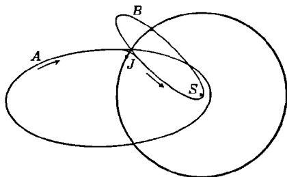
FIG 127 Problem of Three Bodies
