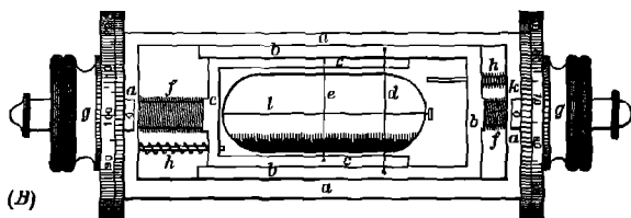
FIG 32 The Filar Position Micrometer
