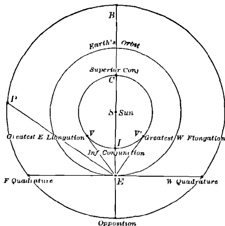
FIG 109 Planetary Configurations
