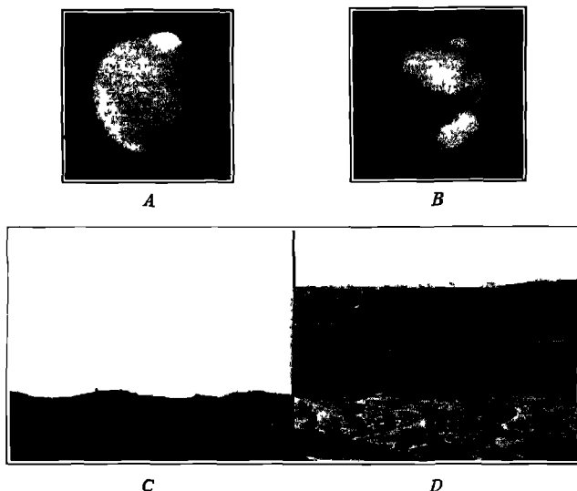
FIG 144 Mars (September 11) and San José as photographed from Mt Hamilton A and C, with violet light B and D with infra red light The occultation in C is due to the earth's atmosphere, and the comparison is suggestive of the presence of an atmosphere of considerable density on Mars San José is distant 13\frac{1}{2} miles from Mt Hamilton G M T of Mars observations A, 18^h 50^m , B, 18^h 30^m
