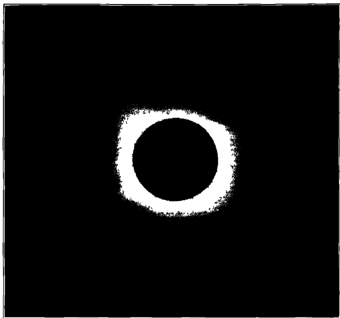
FIG. 97 Eclipse of January 22, 1898, India
