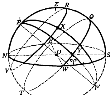
FIG 6 Circles of the Celestial Sphere
