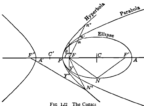
FIG. 122 The Conics
