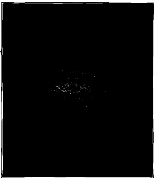
FIG. 153 Shadow-Transit of Ganymede
