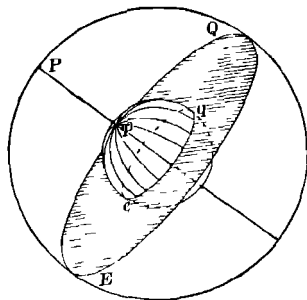
FIG 5 The Plane of the Earth's Equator
