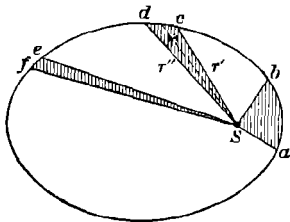
FIG 59 Equable Description of Areas
