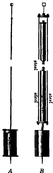
FIG 24 Compensation Pendulums
