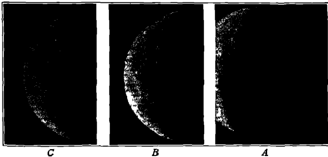
FIG 106 Occultation of Aldebaran, March 22, 1904
