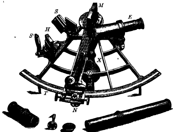
FIG 34 The Sextant
