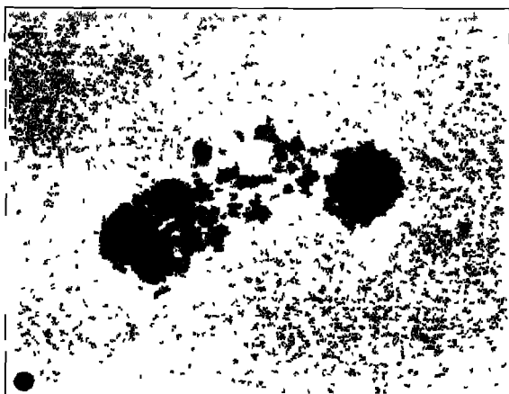
FIG 92 The Great Sun Spot Group of February 8, 1917
