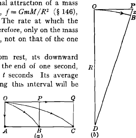
FIG 55 Falling Bodies
