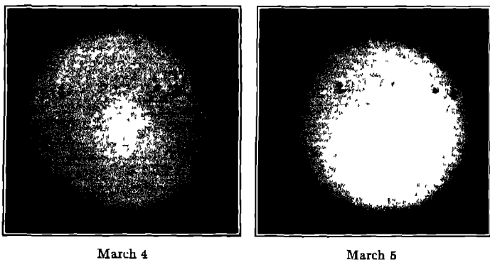
FIG 91 Solar Photographs
