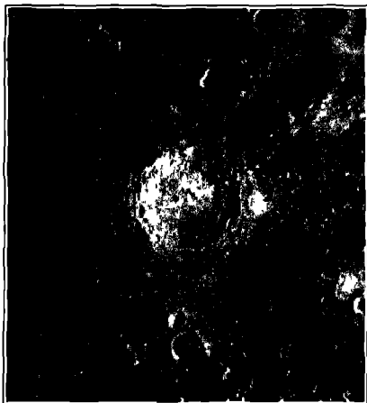
FIG 79 Copernicus
