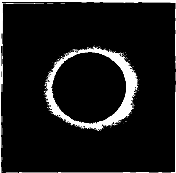
FIG. 104. The Solar Eclipse of January 24, 1925
