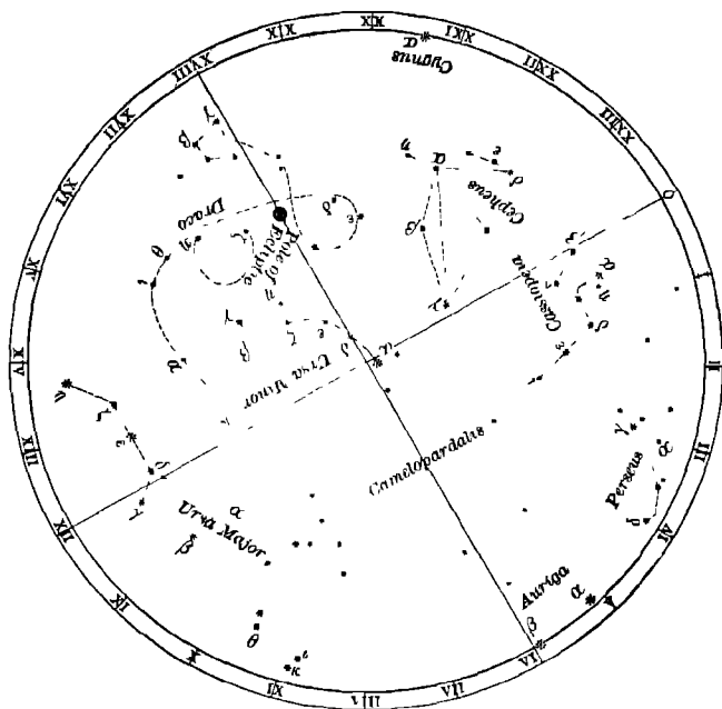
FIG 3 The Northern Circumpolar Constellations
