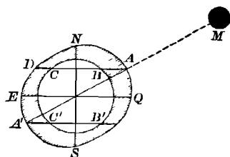
FIG 131 The Diurnal Inequality
