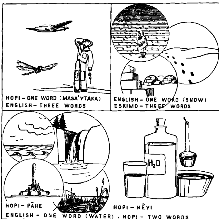
Fig 2 Languages classify items of experience differently The class corresponding to one word and one thought in language A may be regarded by language B as two or more classes corresponding to two or more words and thoughts.
