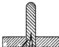
Fig 3 —Method of fixing handle into wooden back-plate.
