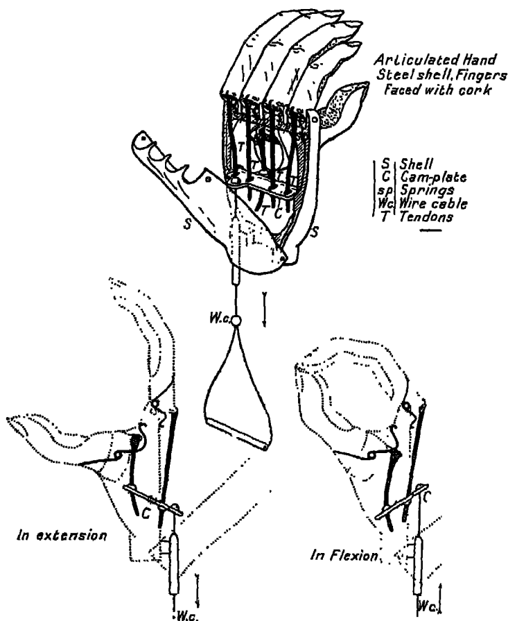
FIG. 104.—Articulated Hand (Caut Type, Amar's Model).
