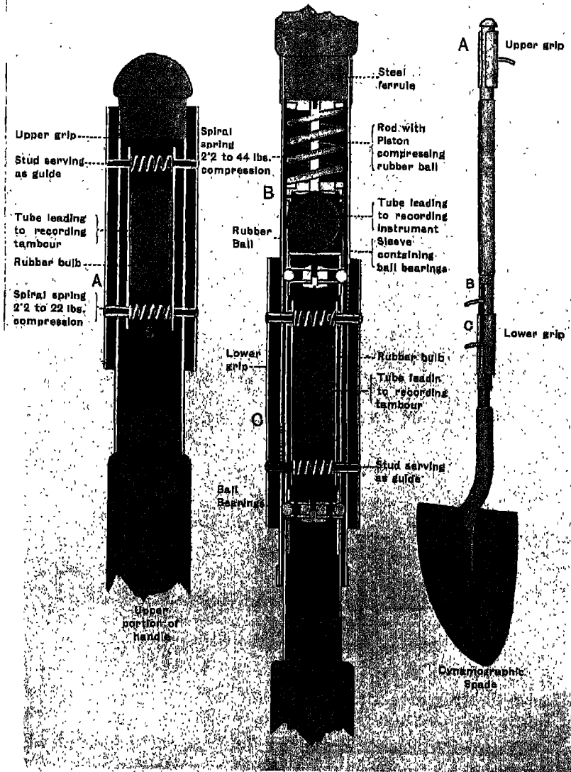
FIG. 24.—Dynamographic Spade (detailed Section.)
