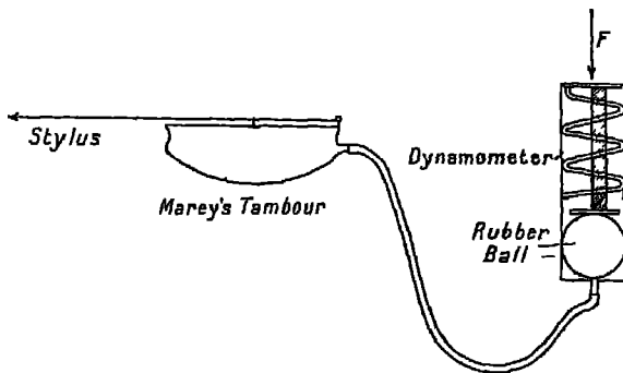
FIG. 19.—Diagram of Recording or Graphic Dynamometer.
