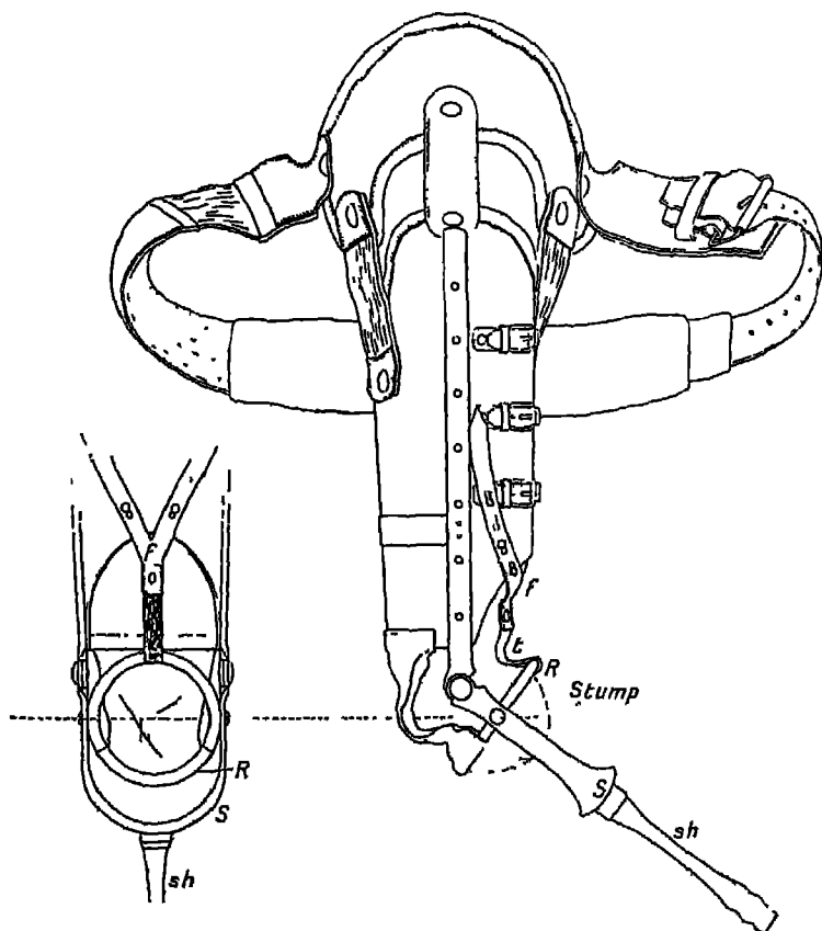
FIG. 102.—Lever Fore-arm (Amat).
