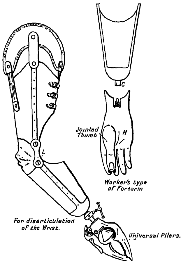
FIG. 101.—Worker's Type of Forearm (Amar).
