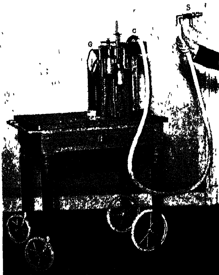
FIG. 26.—Respiration Gauge.
