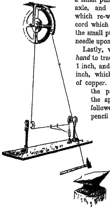
FIG. 122.—Self-registering Hammer.
