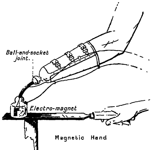
FIG. 103.—Magnetic Hand.
