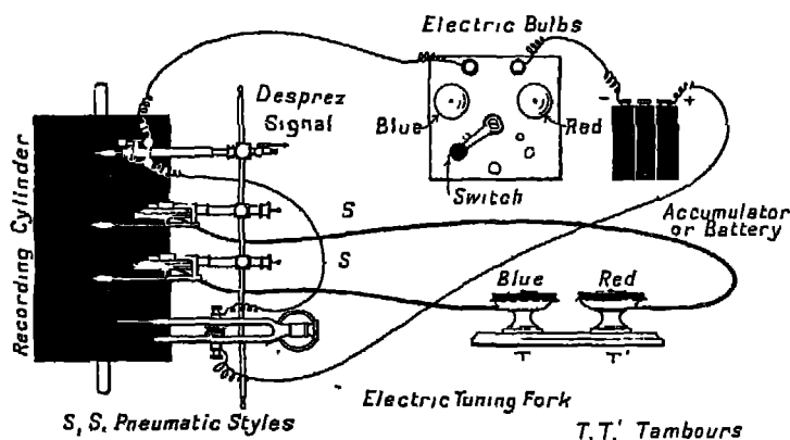
FIG. 18 —Device for Measuring the Personal Equation.
