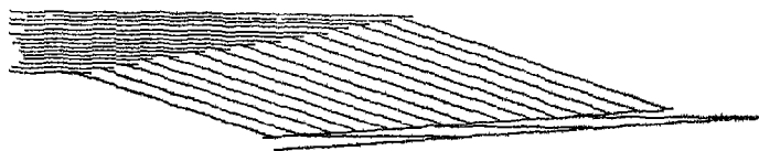
Deltaic Structure (Gilbert)
