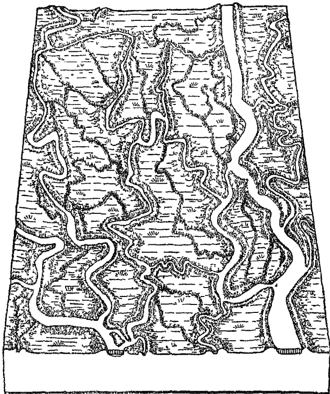
Distributaries and Redistributaries from a Stream
