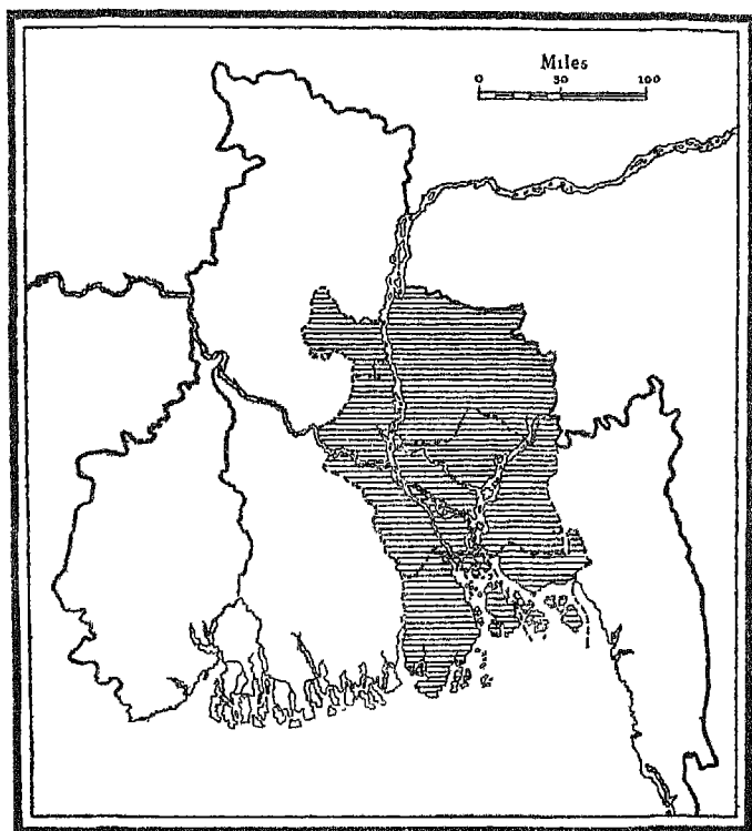
The Bengal Delta (according to S. G. Panandikar)
