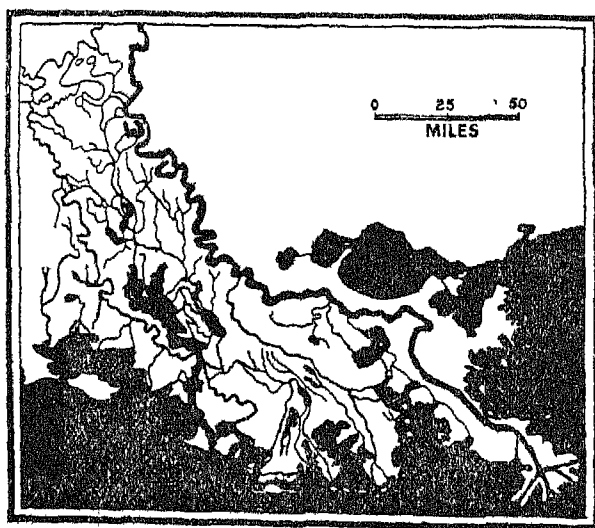
The Mississippi Delta
