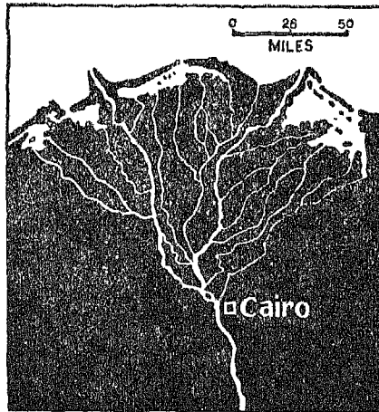
The Nile Delta
