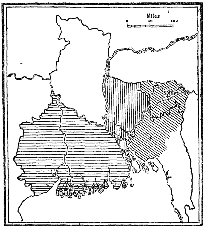
The Bengal Delta (according to R. K. Mukherjee)
