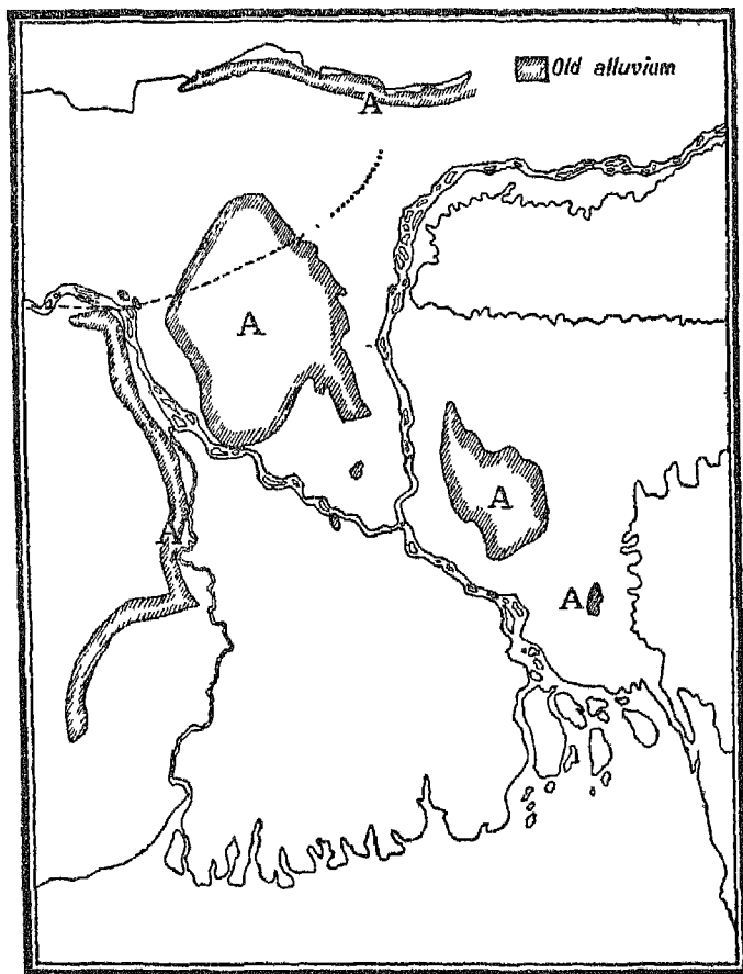
The Ganges Delta (according to Strickland)
