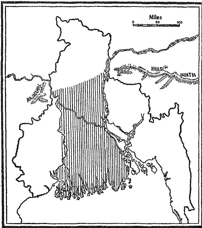
The Ganges Delta (according to Fox)
