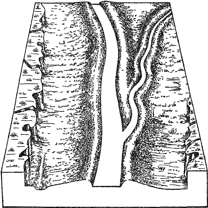
Levees and Shifting Channels
