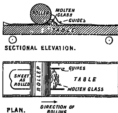
FIG. 11.—Rolling table for rolled plate-glass.
