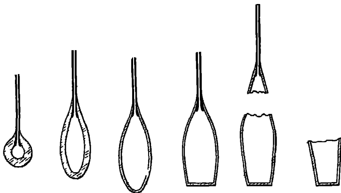
FIG. 10.—Sectional diagram of the evolution of a tumbler.
