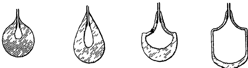
FIG. 14.—Early stages in the formation of cylinders for sheet-glass.
