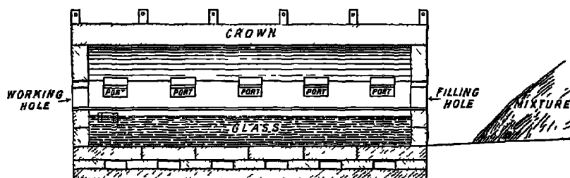
Fig. 8.—Longitudinal sectional diagram of tank furnace.
