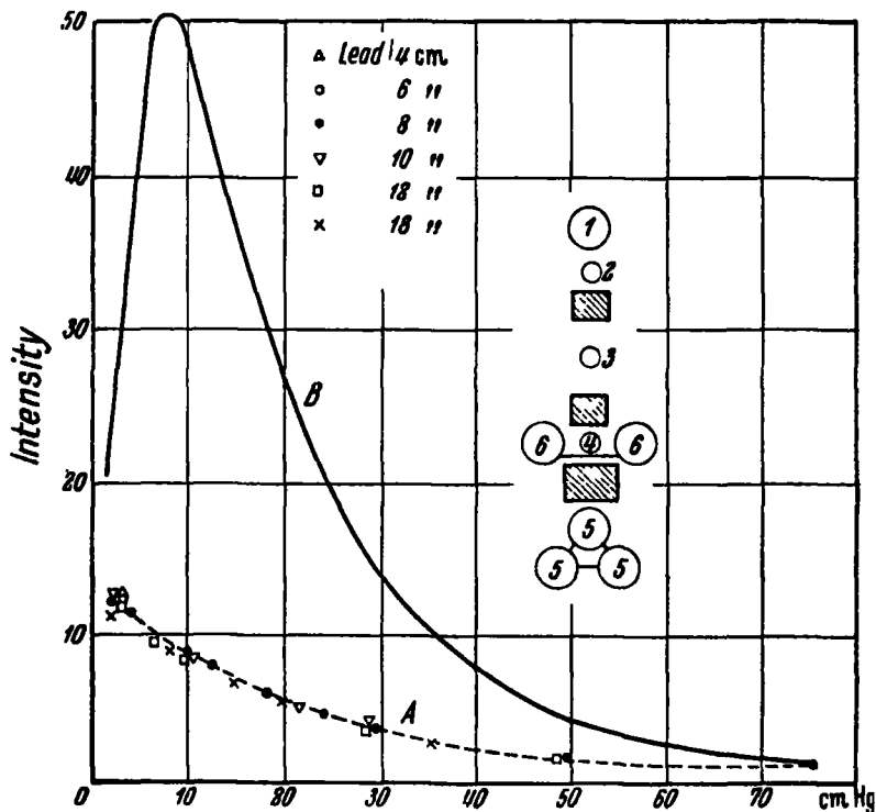
Figure 2 Measurements of SCHEIN, JESSE and WOLLAN (S 5). Curve A: Intensity of the hard component for various thicknesses of lead as a function of pressure in cm Hg. Curve B: Total intensity of cosmic rays according to PROTZER (P 2, 3).
