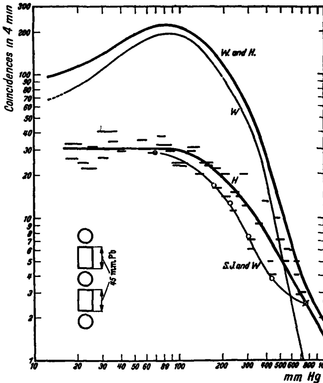
Fig. 1 The number "H" of particles penetrating 9 cm of lead as a function of atmospheric pressure as measured by EHMERT (E 2) with the countertube arrangement sketched in the lower left. The circles and "S J & W" give the measurements of SCHEIN, JESSE, and WALLAN (S 5) with 8 cms of lead. "W & H" shows the variation of the total vertical radiation according to PROTZER (P 2, 3). "W" is the difference of the curves "W & H" and "H" which at the same time agrees with the variation of the shower frequency according to REGNER and EHMERT (R 2).
