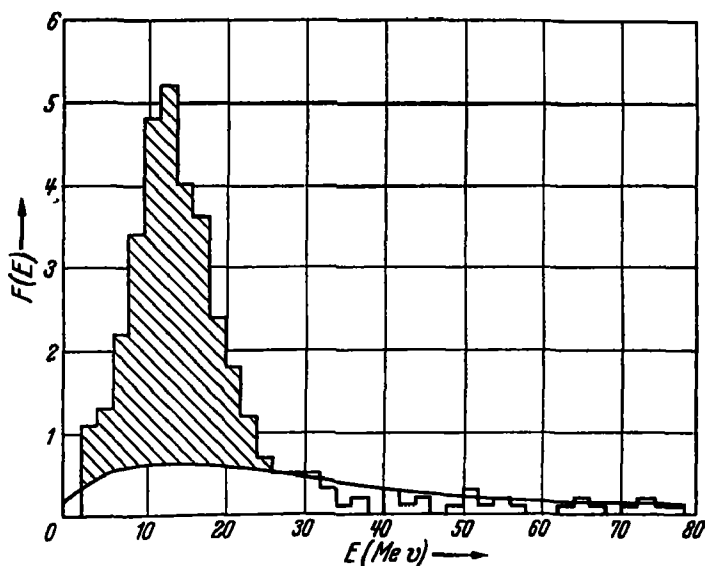
Figure 7 Energy distribution of single proton tracks Step curve Measurements of WIDHALM Smooth curve Theoretical curve F(E)dE
