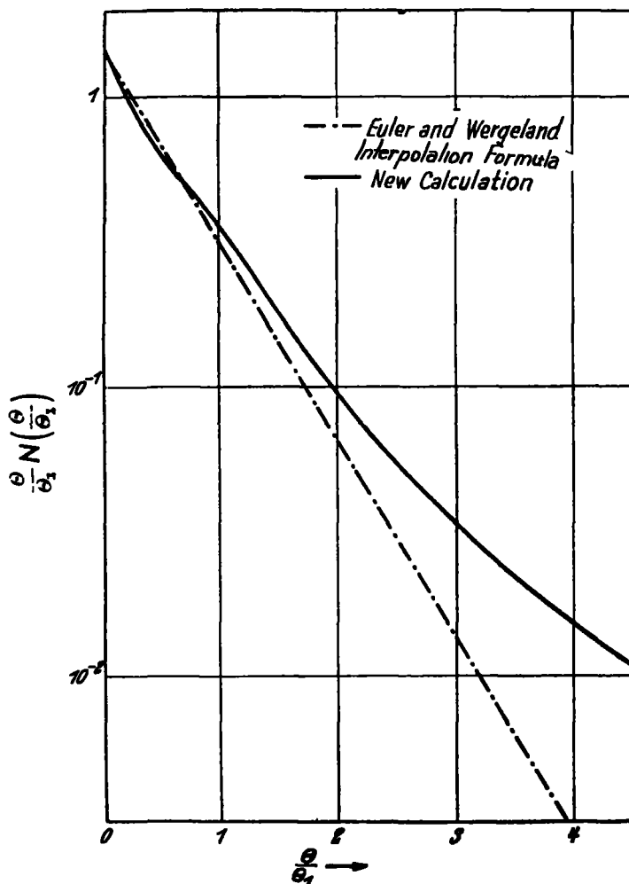
Fig. 1a Angular distribution of shower electrons
