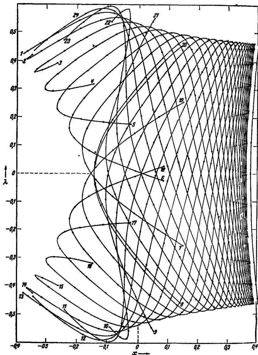
Figure 4 Family of asymptotic orbits for \gamma_1 = 0.85 (According to BARNOS (B 2))
