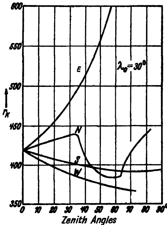
Figure 9. Critical energies (expressed in 10^{10} ) for the north-south and the east-west asymmetries. Positive particles, northern hemisphere. The rise of the N-curve for large zenith angles is due to the simple shadow cone (According to LEMAITRE and VALLARTA (L 9)).
