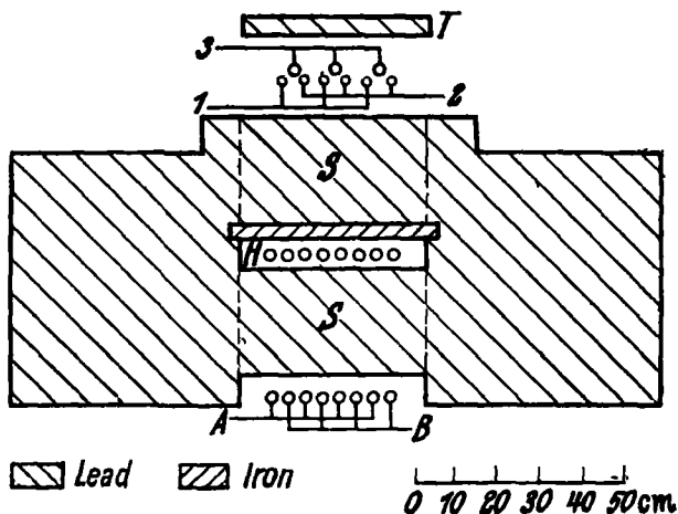
Figure 2 Experimental arrangement of JÁNOSY and INGLEY
