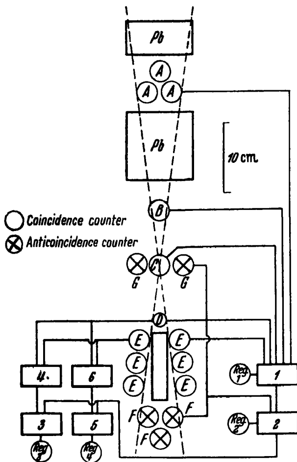
Figure 1 RASSETTI'S arrangement for measuring the decay time of the meson
