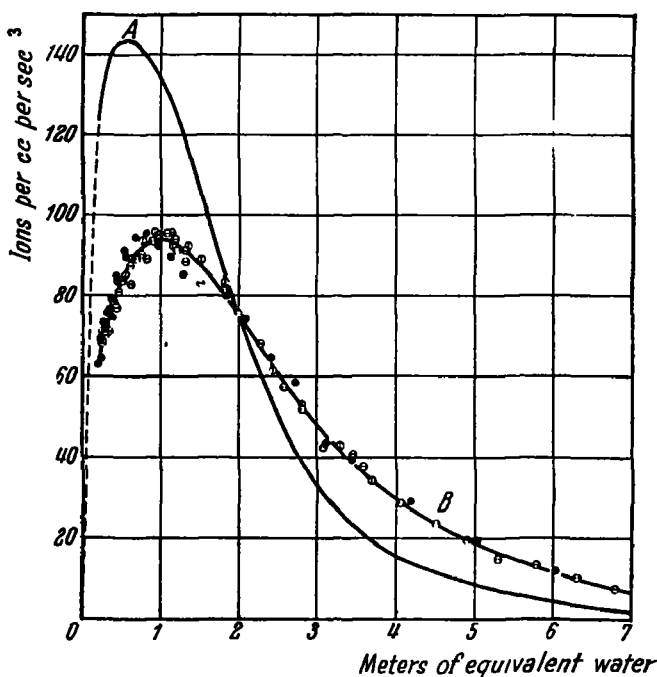
Fig 1 Intensity of the cosmic radiation as a function of the thickness of the air layer passed through, according to BOWEN, MILLIKAN and NIELER. Curve B Intensity in Madras ( 3^\circ north magnetic latitude). Curve A Difference of intensities in Fort Sam Houston ( 38.5^\circ north latitude) and Madras.
