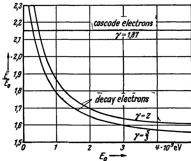
Figure 4. The mean energy of cascade electrons and the decay electrons as function of the lower limit E_0 , above which nuclear disruptions can be released.
