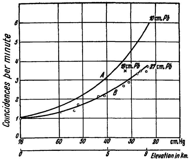
Figure 4 Meson intensity as function of elevation for two different thicknesses of lead absorber
