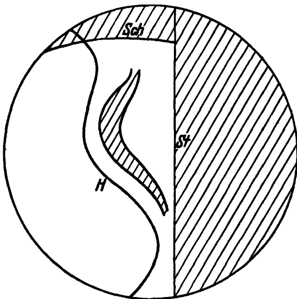
Figure 5. Schematic diagram of allowed and forbidden directions.
