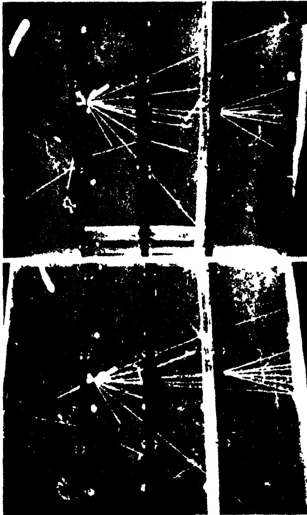
Figure 1 Showers with penetrating particles observed by F. S. FILL
