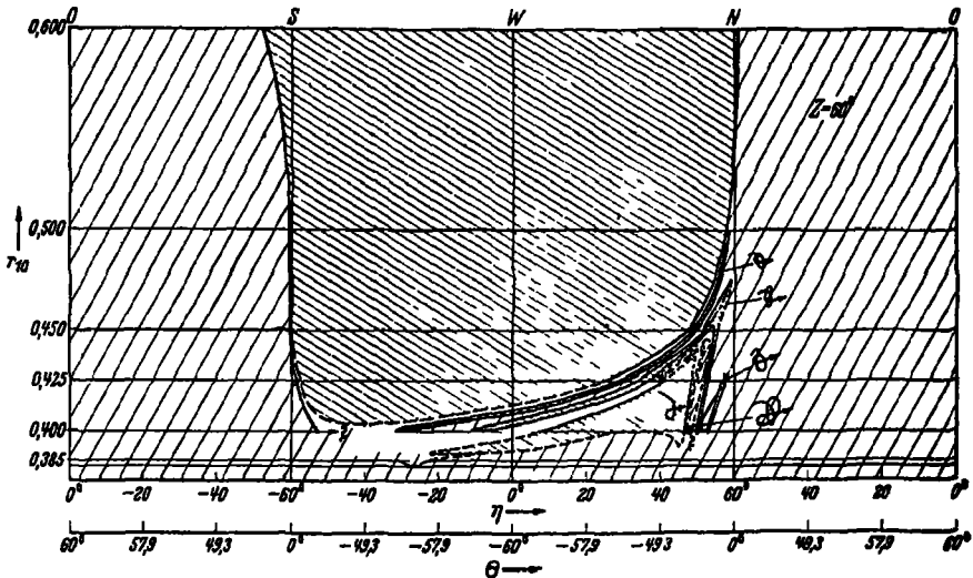
Figure 7 The allowed and forbidden energies (expressed in r_{10} ) at zenith angle z = 60^\circ for various azimuths. The orbital type is given by the figures at the right of the allowed strips. Positive particles, northern hemisphere (According to HUTNER (II 16)).
