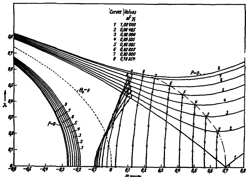
Figure 1 Curves P = 0 , inner stable and outer unstable periodic orbits for various values of \gamma , (according to BAÑOS, URRIBE, and LIFSCHITZ (B 5))
