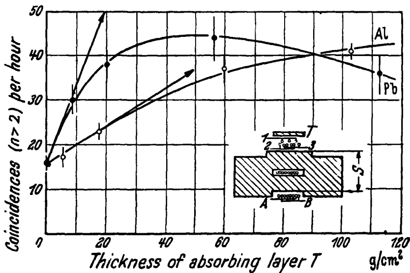
Figure 3 Development of penetrating showers
