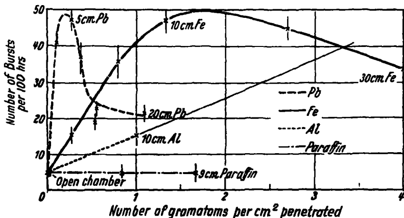
Figure 1. Burst yield curve for Pb, Fe, Al and paraffin. Only bursts > 4 MeV (according to NIE).
