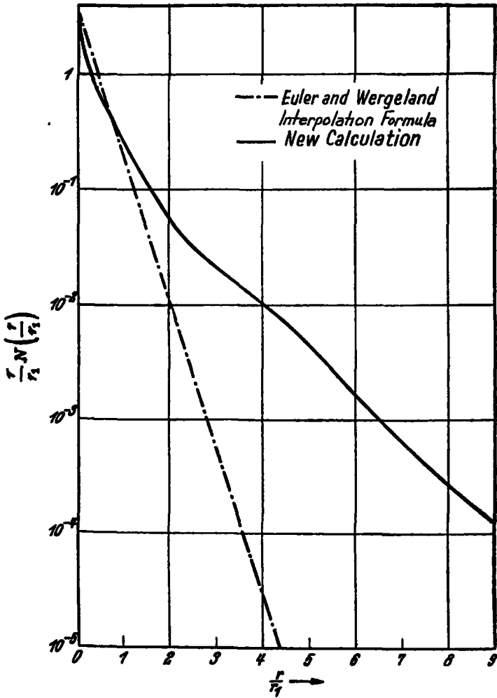
Fig 1b Spacial distribution of shower electrons
