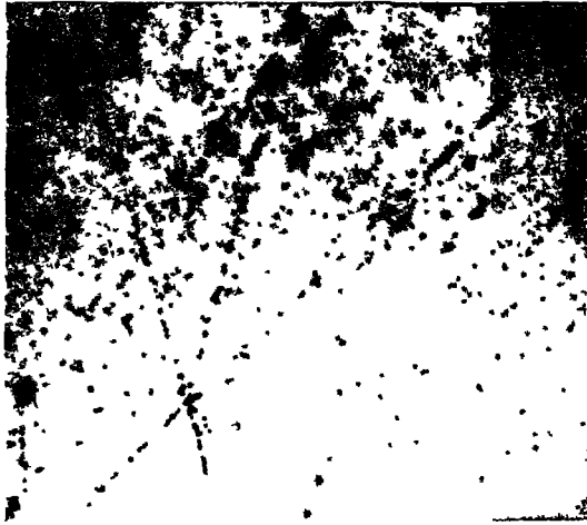
Figure 1 Example of a nuclear disruption in the photographic emulsion
