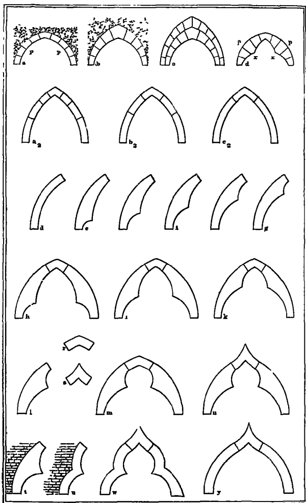
PLATE III. ARCH MASONRY.
