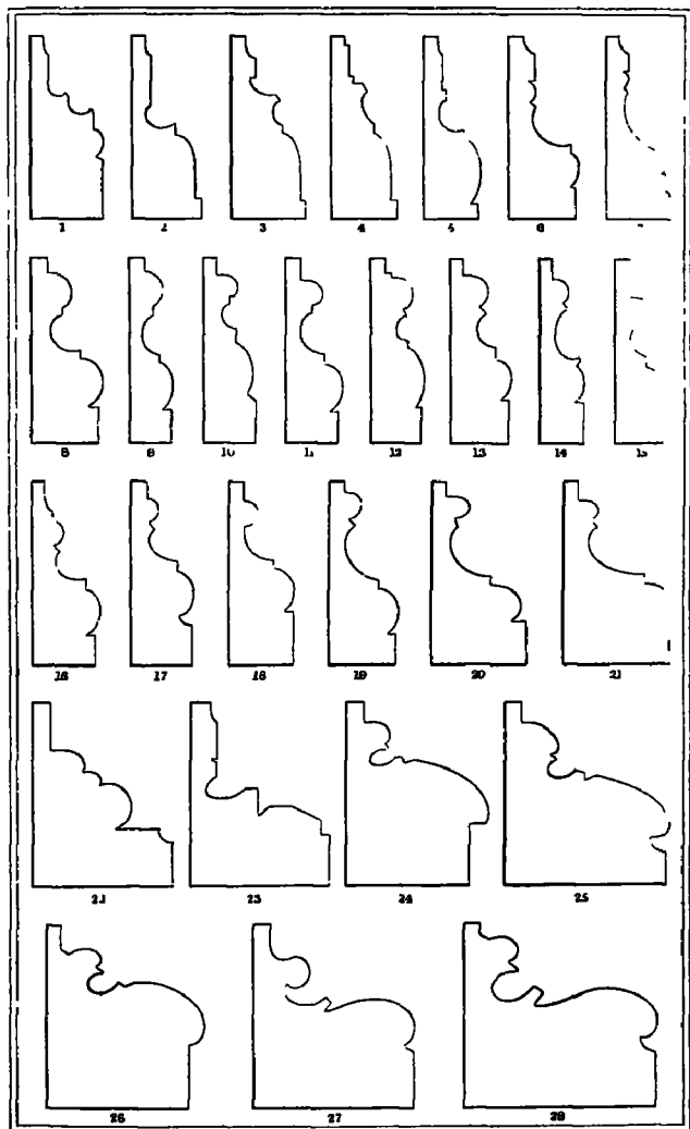
PLATE X. PROFILES OF BASES.
