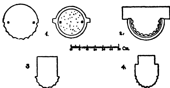
FIG. 72.—Horizontal Sections of Proscenium Columns at Megalopolis and Eretria (1), Epidaurus (2), Delos (3), and Oropus (4).
