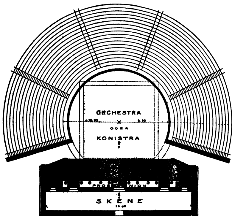
FIG. 58.—Ground Plan of the Graeco-Roman Theater at Termessus
