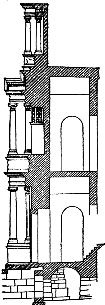
FIG. 24a.—Cross-Section of the Proscenium ( Bühnenfassade ) of the Graeco-Roman Theater at Ephesus according to Hörmann.
