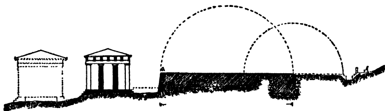
FIG. 32a.—Cross-Section of Precinct of Dionysus Eleuthereus in Athens, Showing Later and Early Temples and Early Terrace and Later Orchestra.
