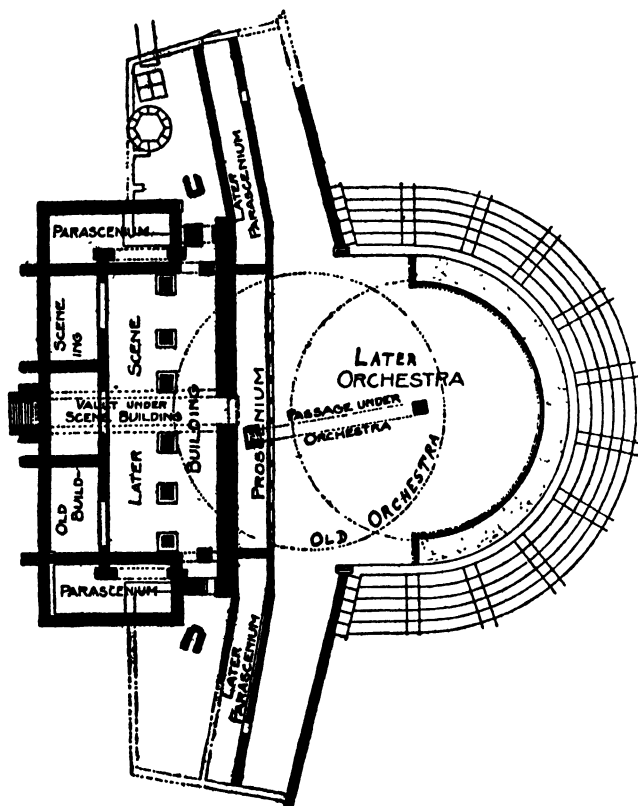
FIG. 53.—Ground Plan of the Theater at Eretria in Euboea
