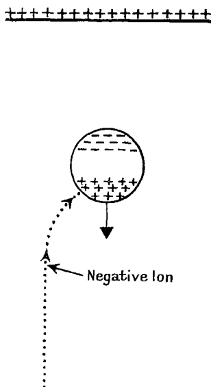
FIG. 22.—Capture of negative ions by large falling drops.
