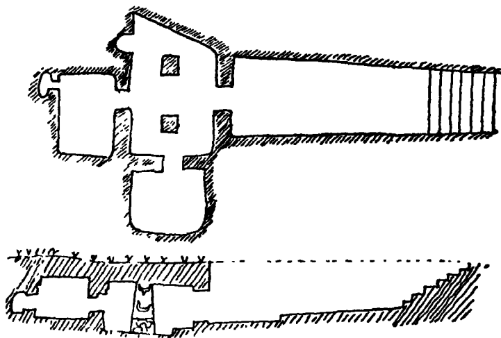
FIG. 7. Megalithic tomb at Anghelu Rujū
