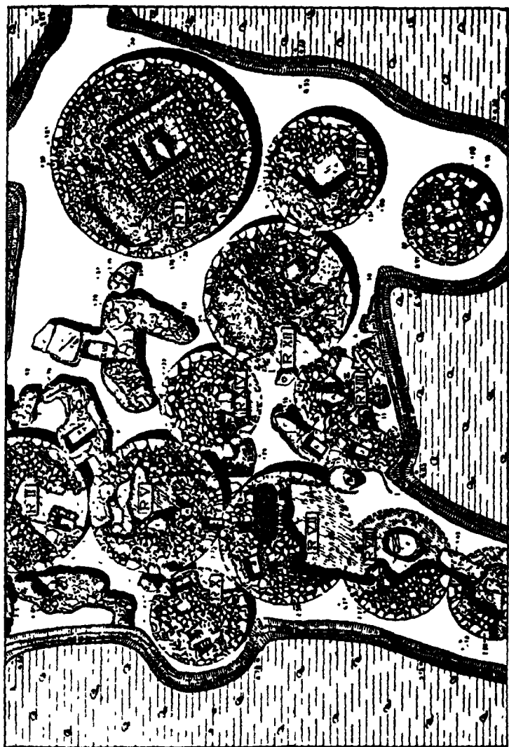
Fig. 1.—Tombs in the island of Lemnos
