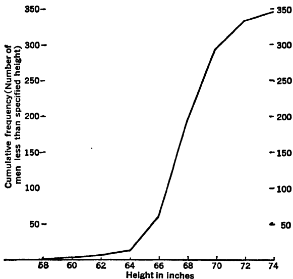
FIG. 3.—Cumulative Frequency Diagram.
