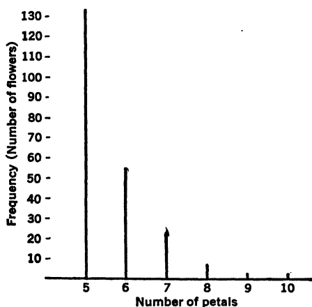
FIG. 2.—Frequency Diagram. Discrete Variable—Number of Petals on a Species of Flower.
