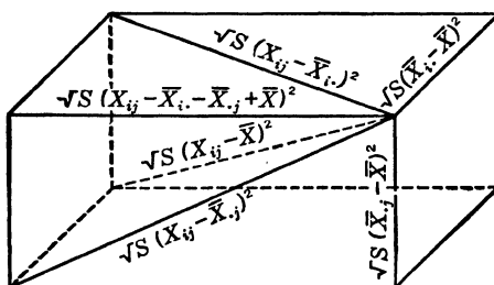
FIG. 11.—Analysis of Variance Diagram.
