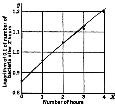
FIG. 7.—Plot of X and y of Table 7.
