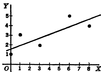
FIG. 5.—Line of Least Squares.
