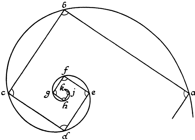
FIG. 3.—Logarithmic Spiral.
