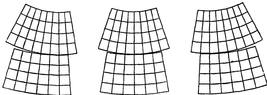
Figure 38.—Rolling contact between charts in adjacent Lambert projection bands.
