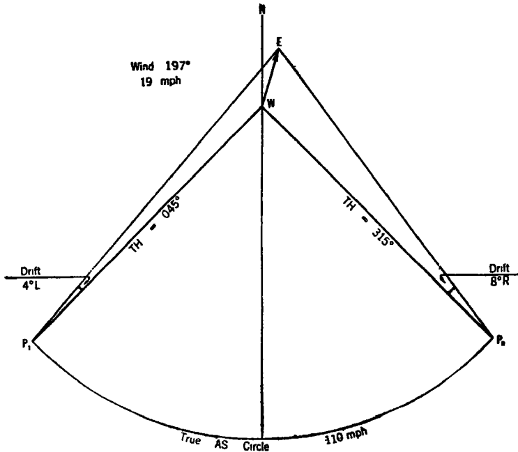
Figure 105.—Graphic plot for determination of wind by double drift method.
