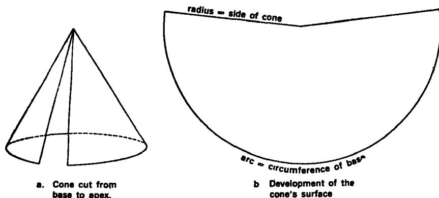
Figure 26.—Development of a conical surface.
