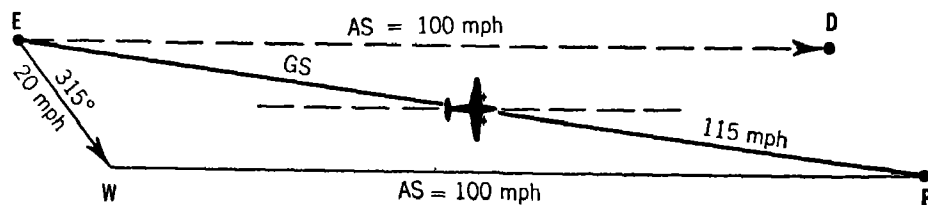
Figure 84.—Wind drift.
