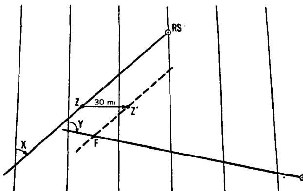
Figure 162 A "running fix" from radio bearings.
