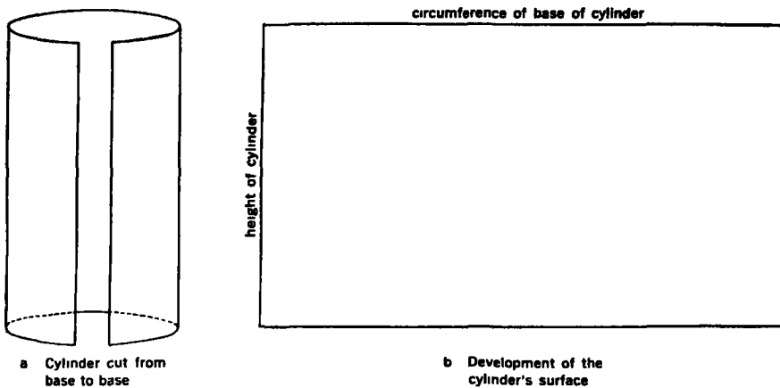
Figure 27 --Development of a cylindrical surface.
