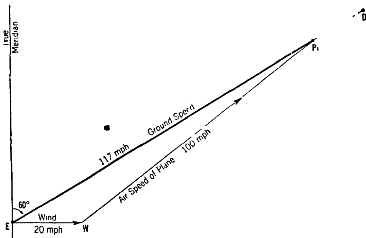
Figure 109.—Radius of action; wind triangle for flight out.
