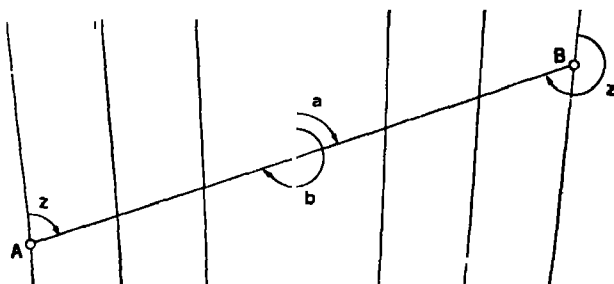
Angle a is the course to be followed from A to B. Angle b is the course to be followed from B to A. Angle z is the bearing, or azimuth, of B as measured at the point A. Angle z is the bearing or azimuth of A as measured at the point B.
