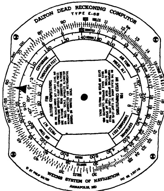
Figure 130.—Finding the correct altitude.
