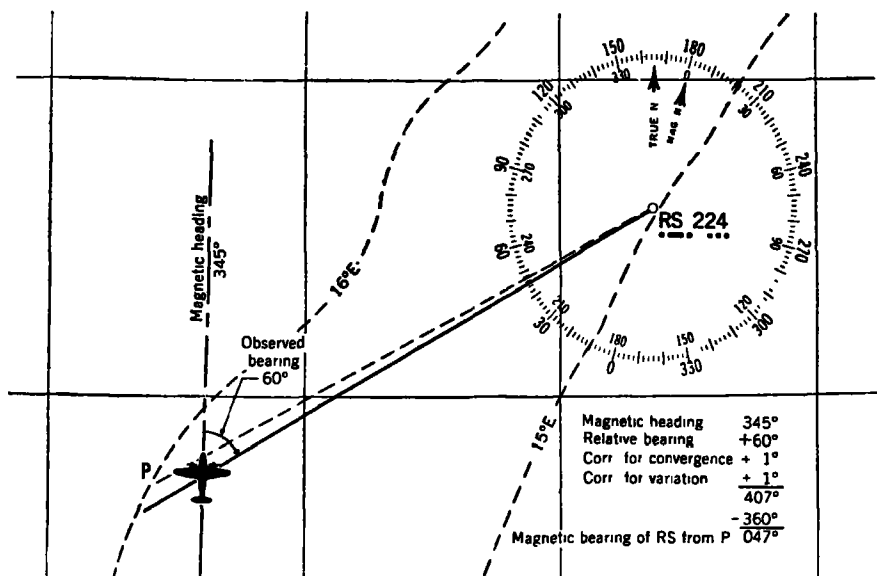
Figure 172.—Bearing and direction finding chart corrected for converge
