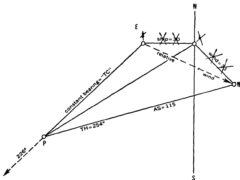
Figure 121 —The "relative wind triangle."
