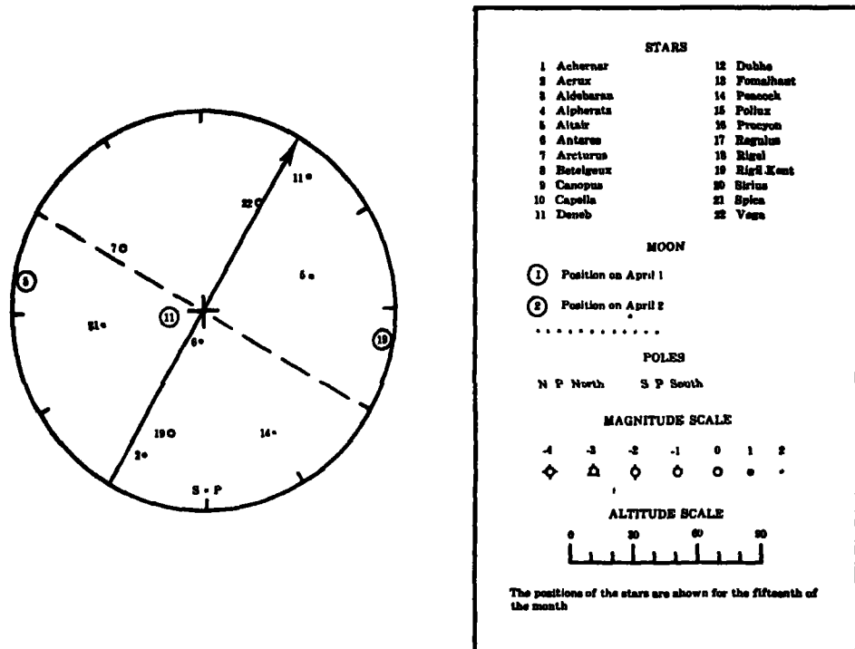
Figure 189.—Sky diagram for latitude 10^{\circ} S., at 0300 LCT, April 1944, with legend.
