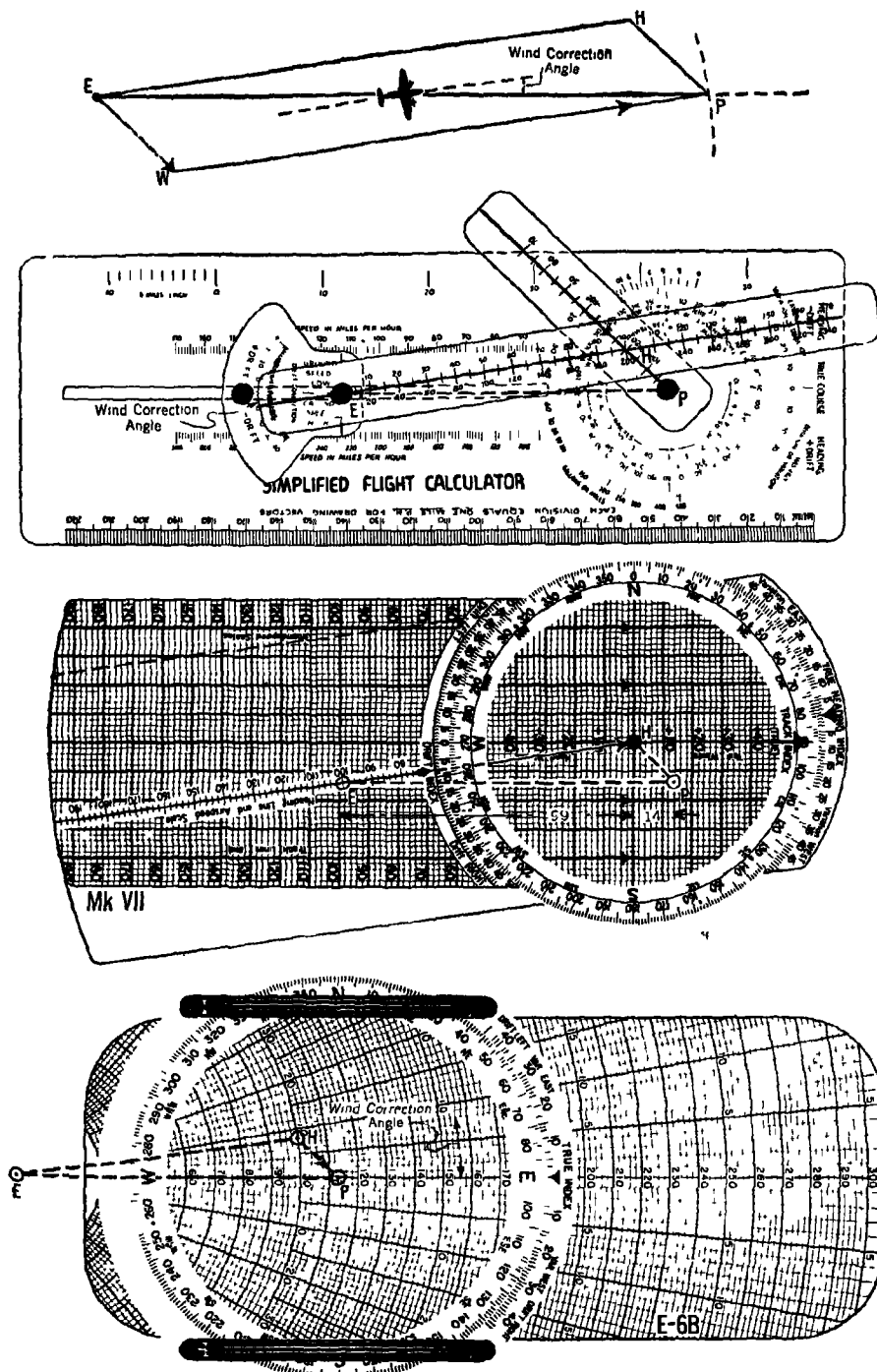
Figure 132—Allowances for wind set up on three computers.
