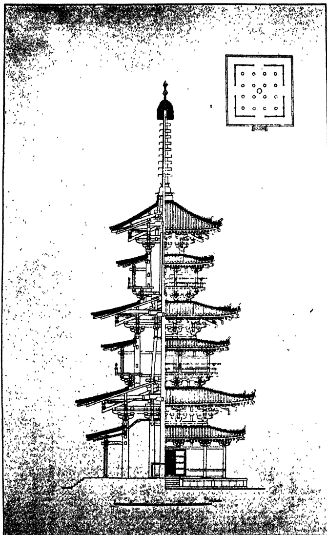
VI SECTION AND ELEVATION OF PAGODA YAKUSHIJI
