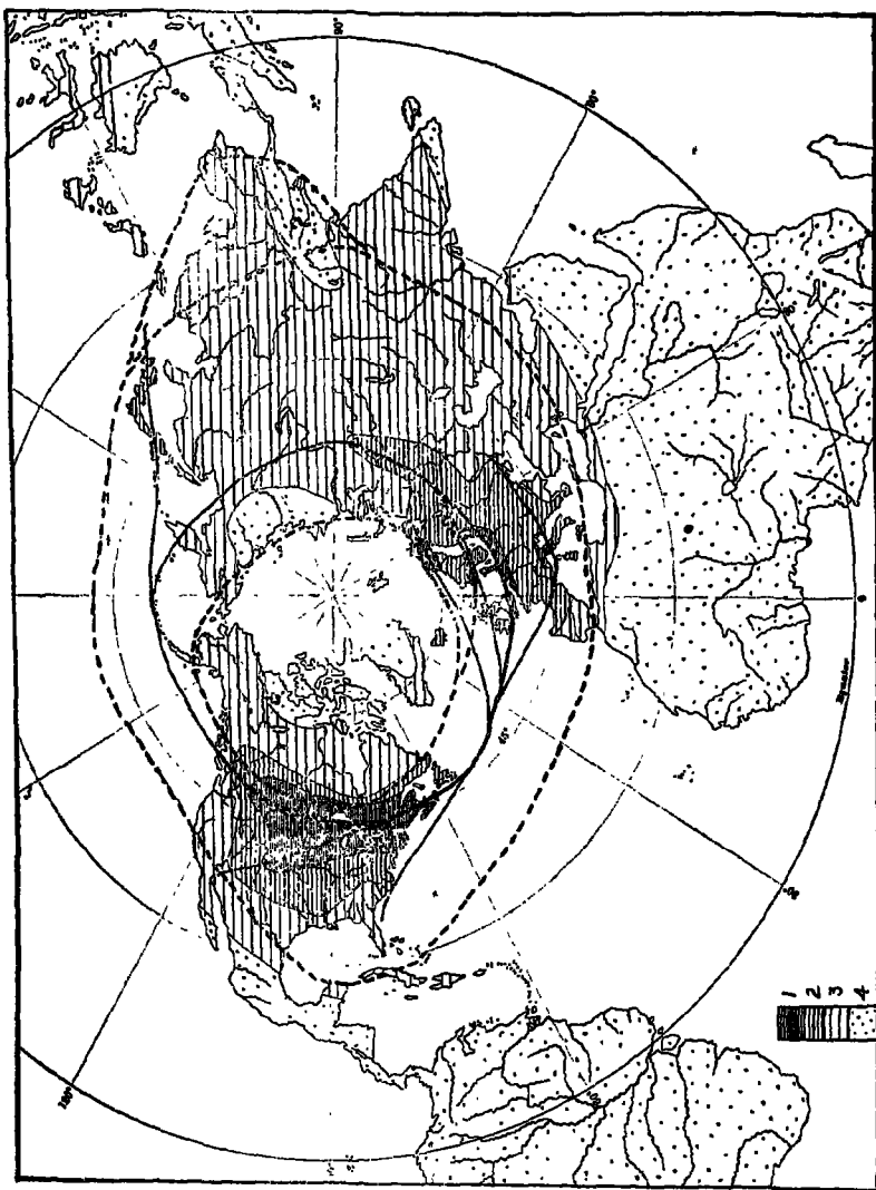
Figure 48. The Shifting of the Storm Belt
