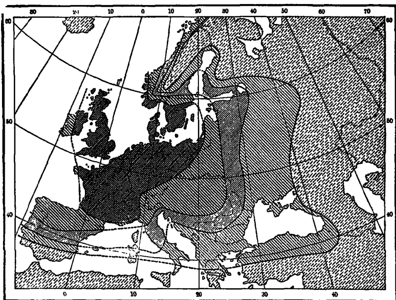
Figure 40. Distribution of Climatic Energy in Europe
