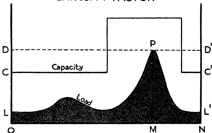
DIAGRAM XIX. LOAD FACTOR AND CAPACITY FACTOR
