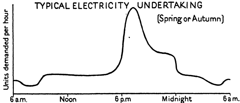
DIAGRAM XXXIII. DAILY LIGHTING LOAD-CURVE OF TYPICAL ELECTRICITY UNDERTAKING
