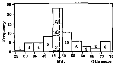
FIG. 22. Illustrating the median for the scores on the Otis Self-Administering Test
