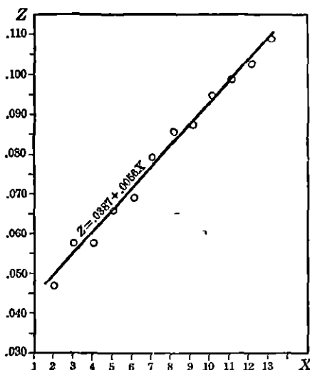
FIG. 72. Illustrating the method of rectifying the hyperbola for Thurstone's data
