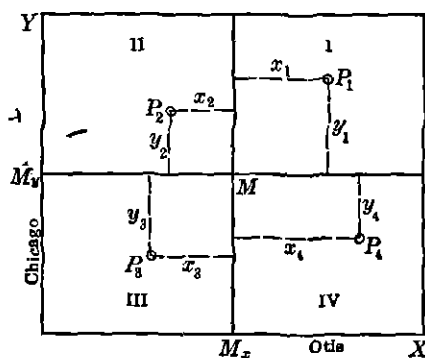
FIG. 38. Illustrating product moments in four quadrants
