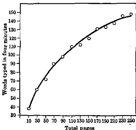
FIG. 73. Thurstone's data fitted with a hyperbola by the method of averages
