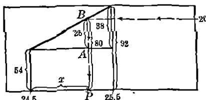
FIG. 30. Enlargement of a portion of the cumulative frequency curve to illustrate the calculation of P_{20}
