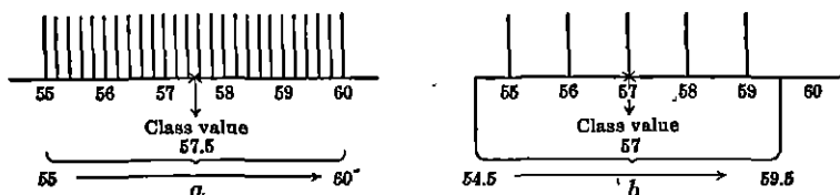
FIG. 5. Illustrating class values and limits with measurements a, very fine; b, to nearest integer
