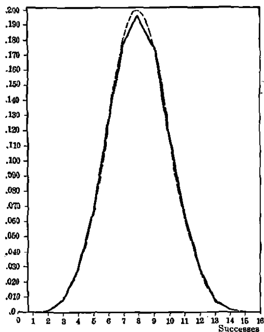
FIG. 54. The point binomial (\frac{1}{2} + \frac{1}{2})^{16} compared with the normal curve
