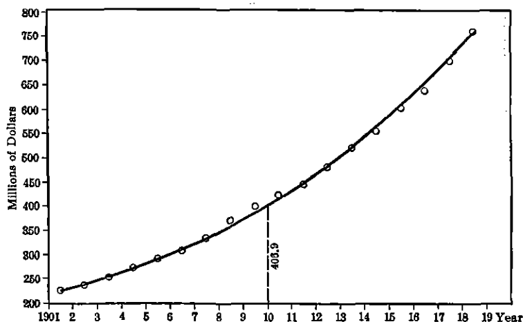
FIG. 24. Plot of the cost data and theoretical series from Table 15
