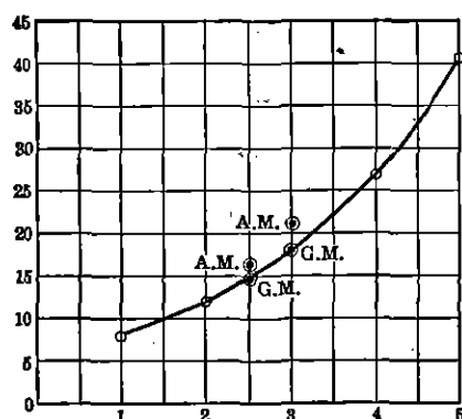
FIG. 23. Illustrating the geometric and arithmetic means for four and five items
