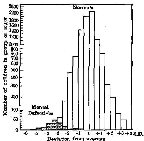
FIG. 49. Distribution according to general intelligence of children of ordinary elementary and special M.D. schools
