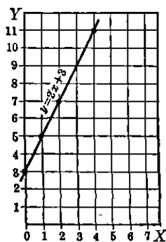
FIG. 15. Graph of y = 2x + 3
