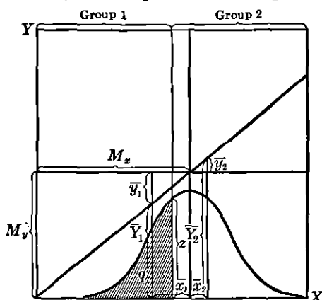
FIG. 68. Illustrating biserial r
