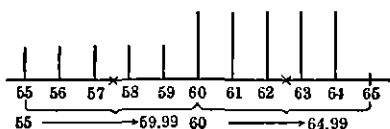
FIG. 3. Illustrating the incorrect class limits which appear when the items are measured to the nearest integer
