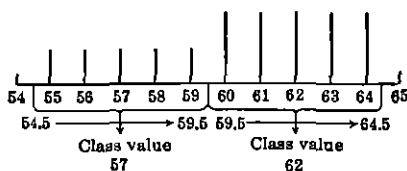
FIG. 4. Illustrating the correct method of stating class limits when the items are given to the nearest integer
