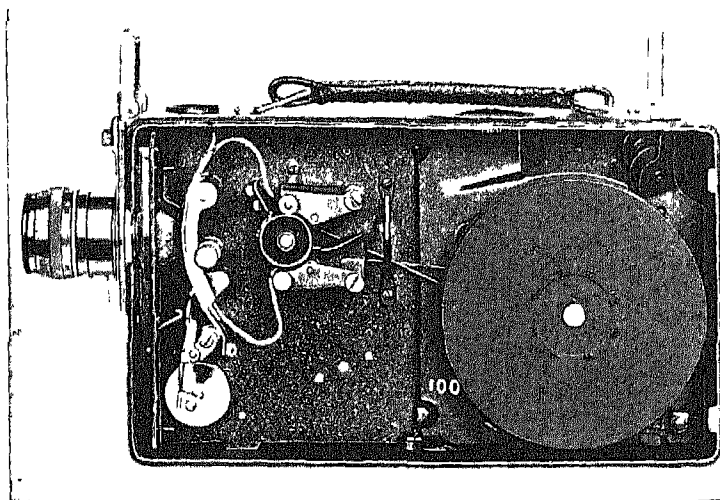
FIG. 6. The internal mechanism of a motion-picture camera. (Eastman Kodak Co)
