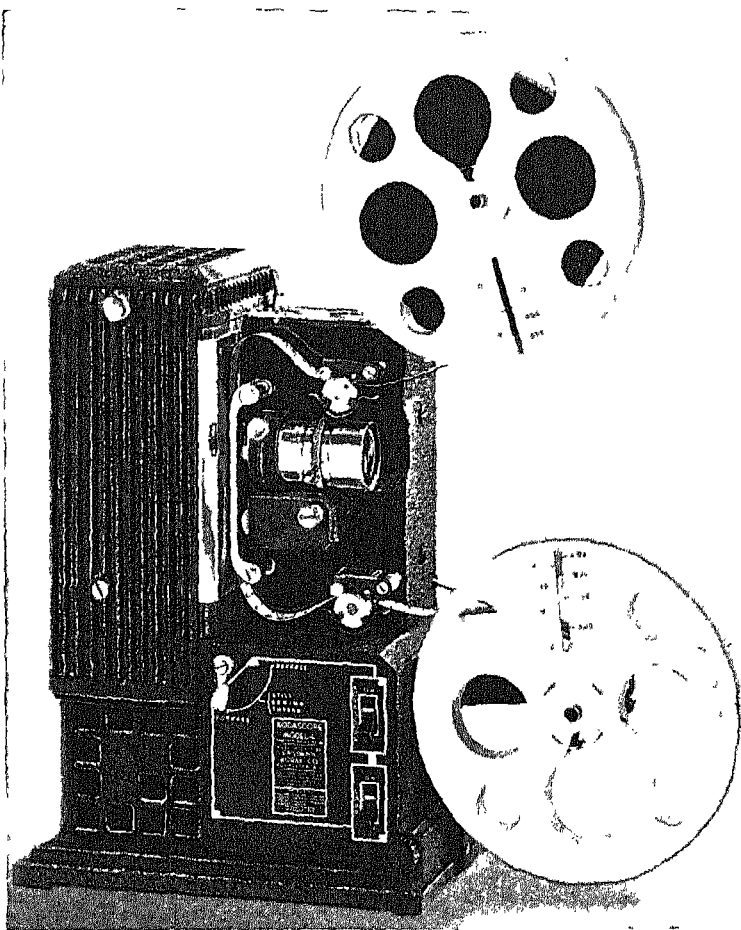
FIG. 25. A 16 mm. silent projector. (Eastman Kodak Co.)
