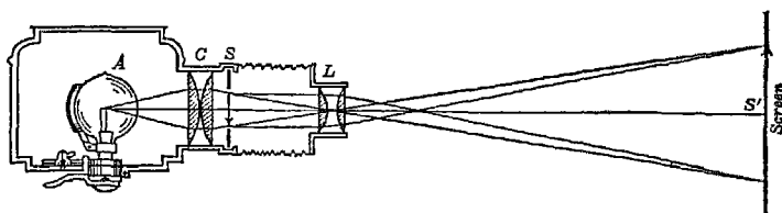
FIG. 17. The construction of a projector. A , incandescent lamp; C , condenser; S , picture carrier; L , objective lens; S' , screen. (From Black, Introduction to College Physics .)
