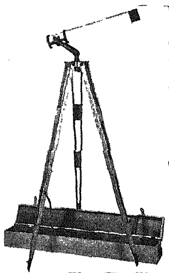
FIG. 16 A portable telescope. (Bausch and Lomb Optical Co.)
