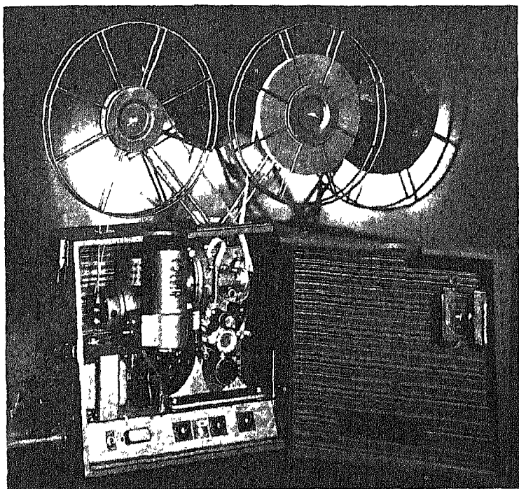
FIG. 27. A 16 mm. sound-film projector. (Victor Animatograph Corp.)
