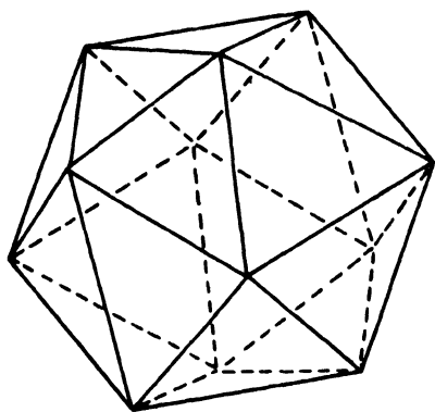
PLATE VIII The Five Regular Solids
