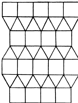
PLATE XX Two Regular Partitions of the Plane
