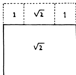
PLATE XLVII The \sqrt{2} Rectangle, Harmonic Decompositions
