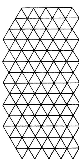
PLATE XIX Regular Equipartitions of the Plane
