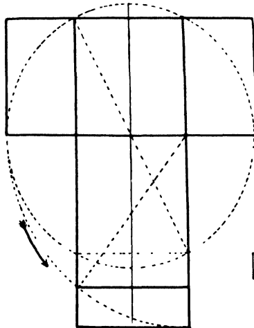
PLATE XLIX The \sqrt{5} Rectangle, Harmonic Decompositions
