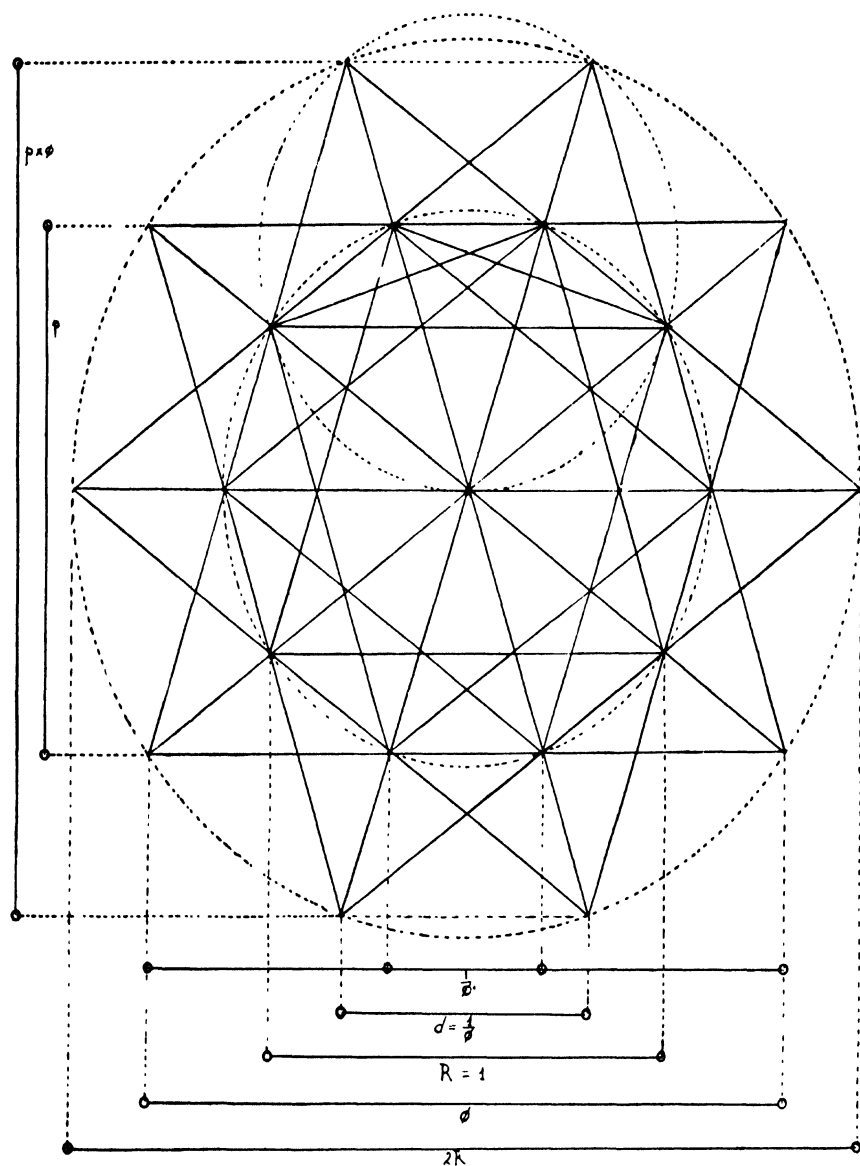
PLATE VII Interplay of Proportions between Pentagon, Pentagram, Decagon and Star-Decagon
