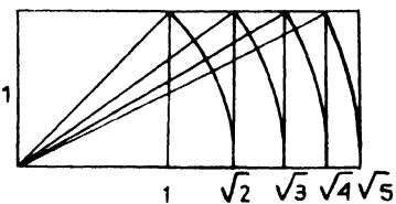
PLATE XLVI Static and Dynamic Rectangles
