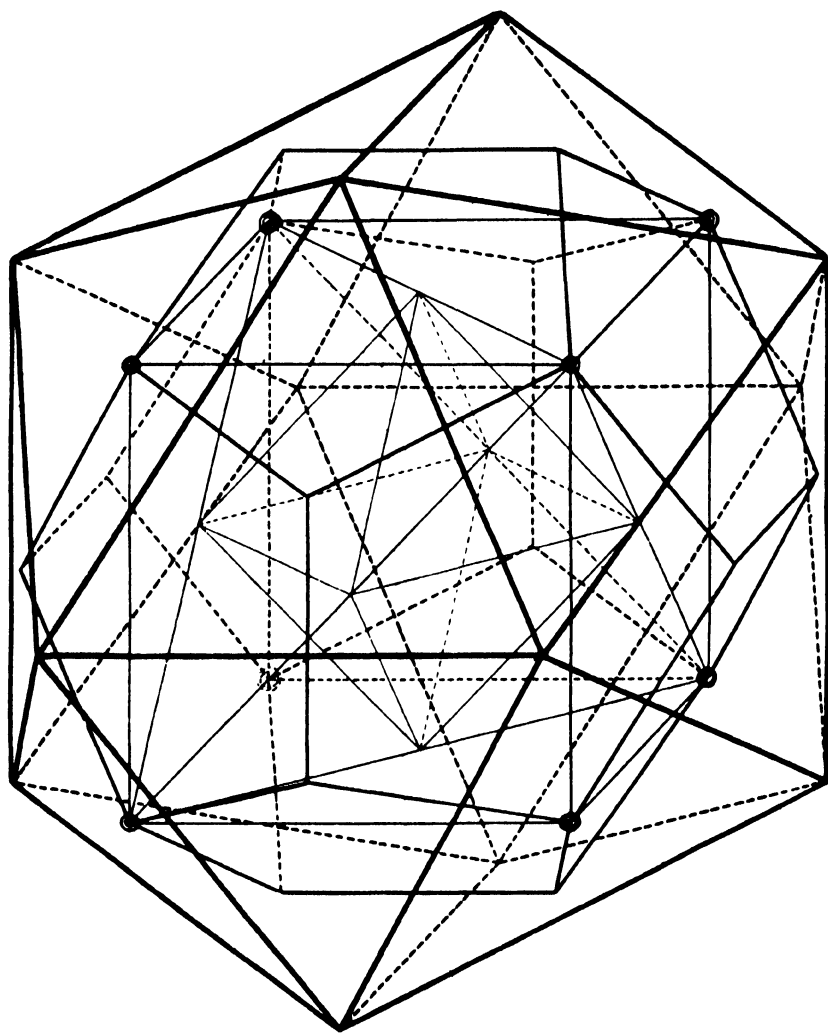
PLATE IX The Five Regular Solids Inscribed within Each Other
