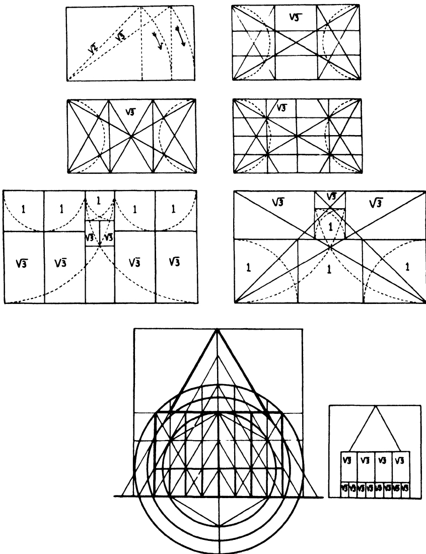
PLATE XLVIII The \sqrt{3} Rectangle, Harmonic Decompositions
