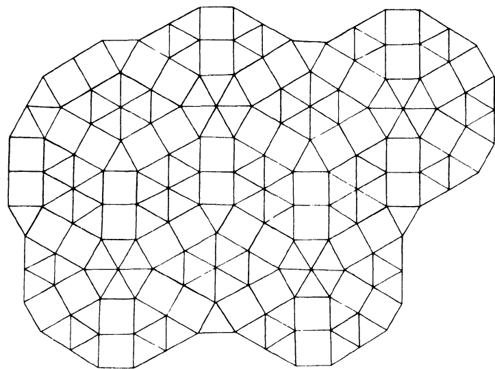
PLATE XXVI Semi-Regular Partition of the Plane
