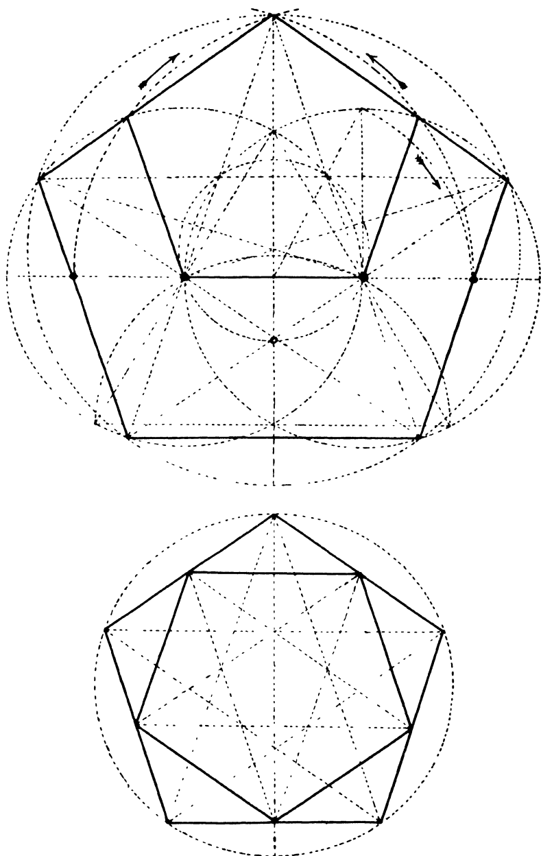
PLATE V Construction of the Pentagon of Given Sides Pentagon and Pentagram
