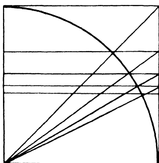
PLATE XLVI Static and Dynamic Rectangles
