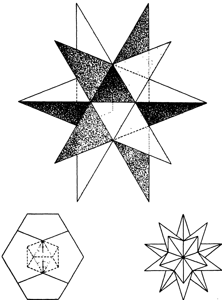
PLATE X Star-Dodecahedron with Twenty Vertices
