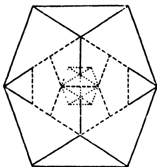
PLATE XI Star-Dodecahedron with Twelve Vertices
